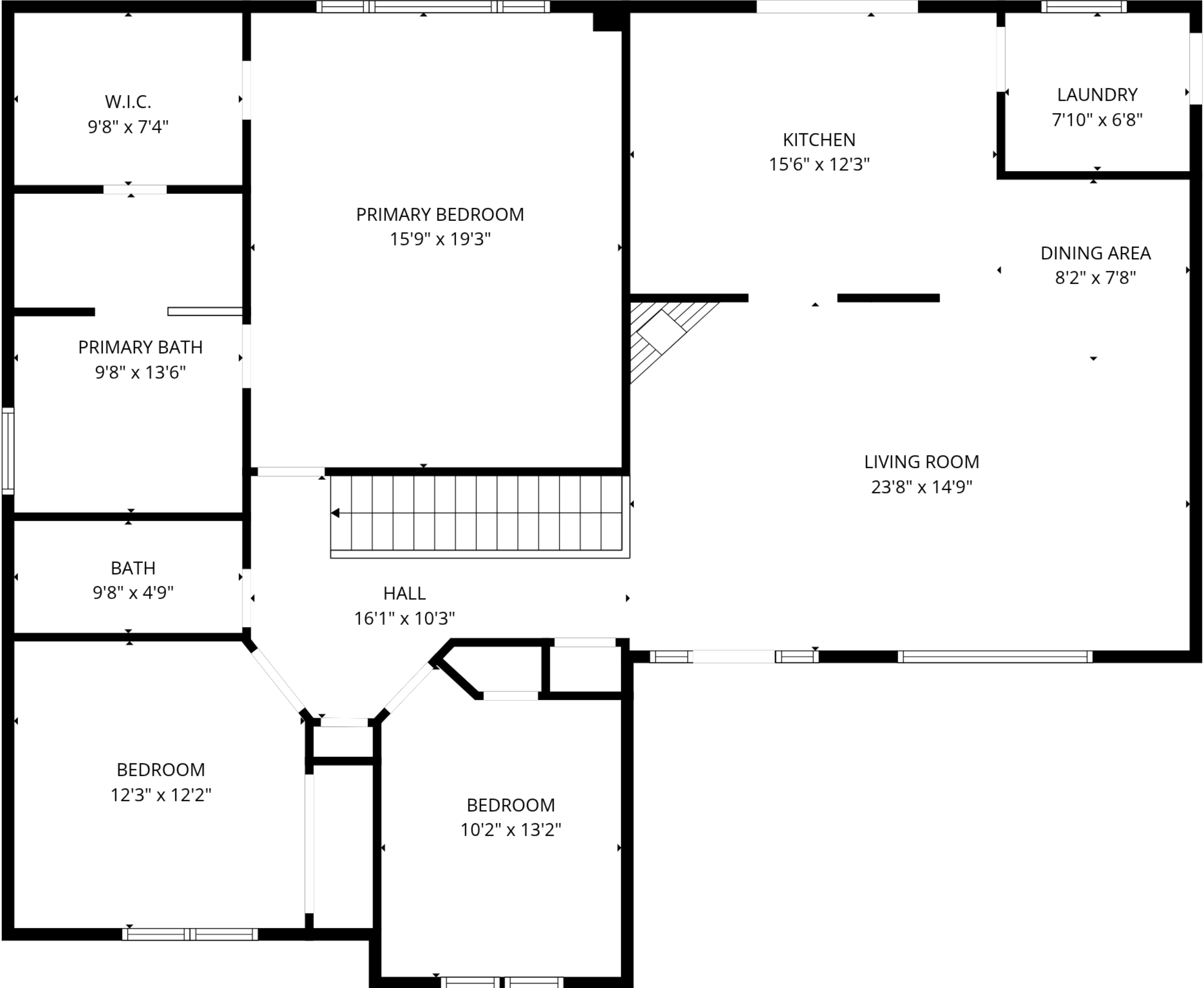
FLOOR 2
