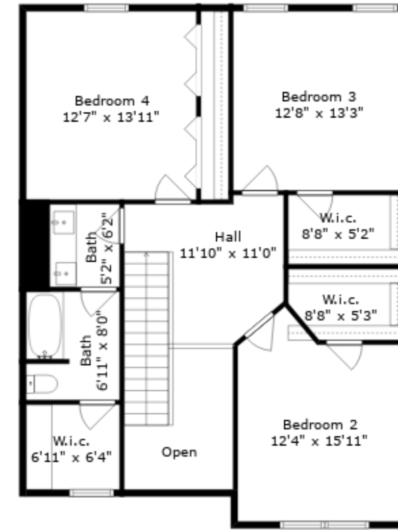
Upper Floor
