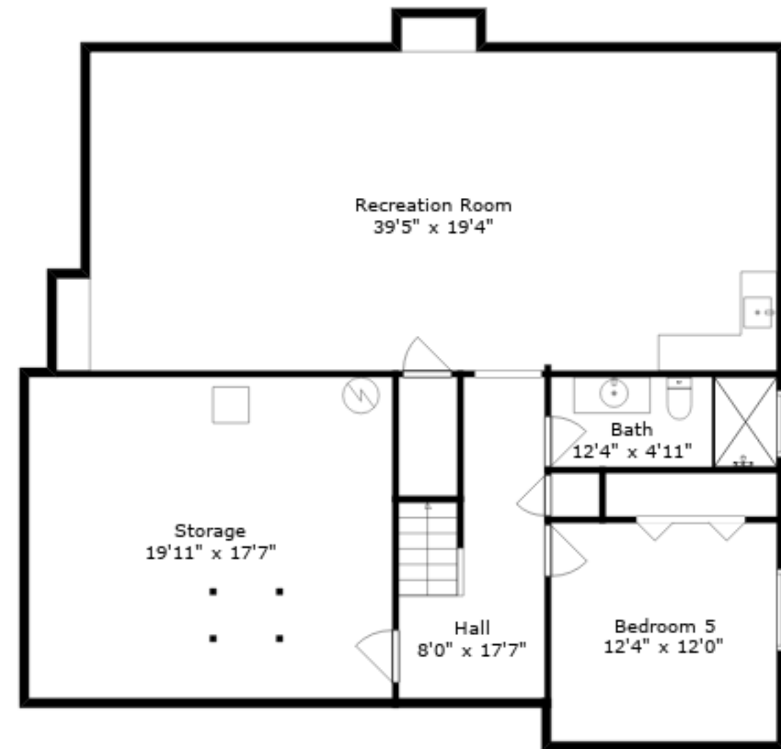
Lower Floor
