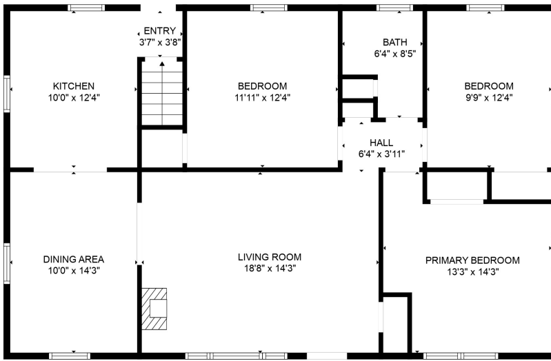
FLOOR 2
