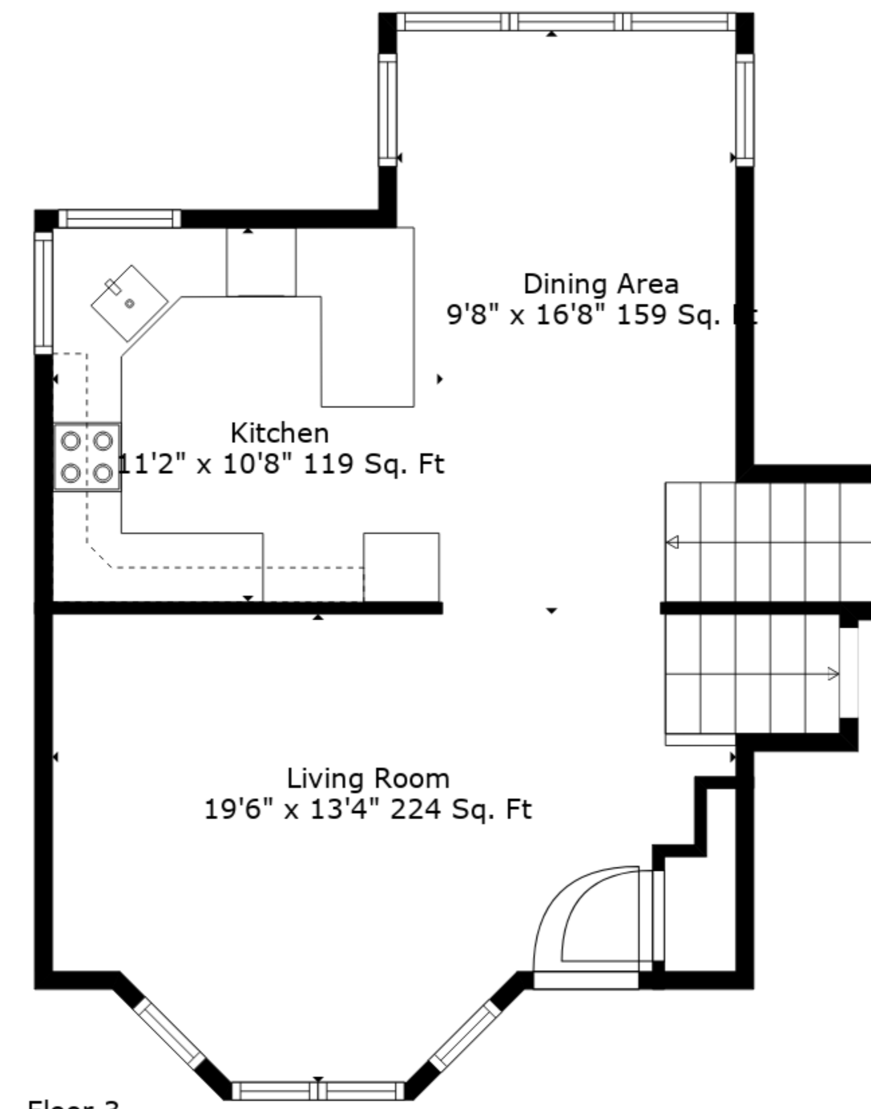
Floor 3
