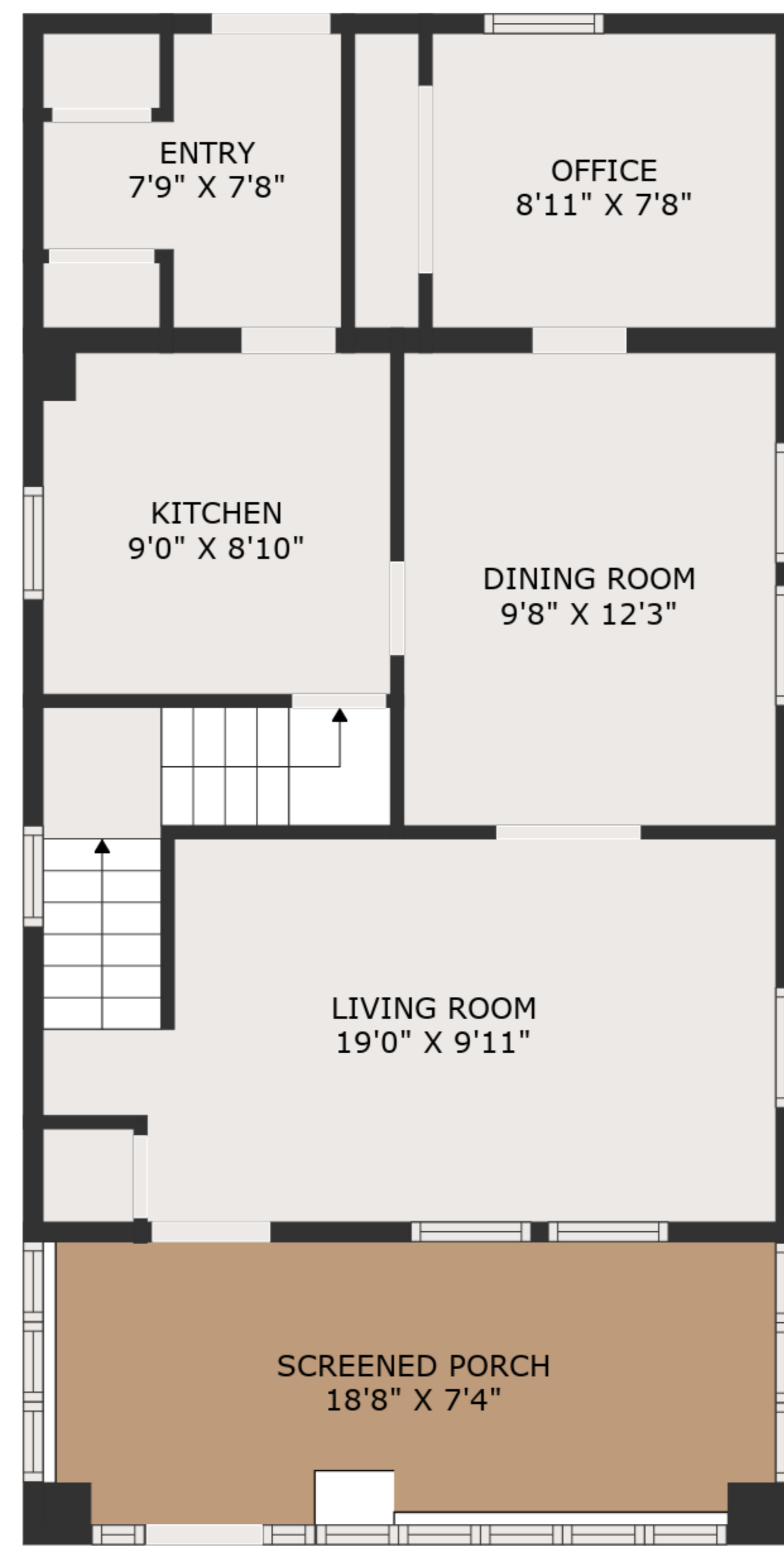
FLOOR 2
