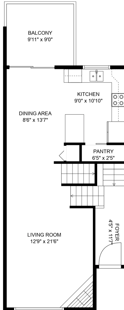
FLOOR 2
