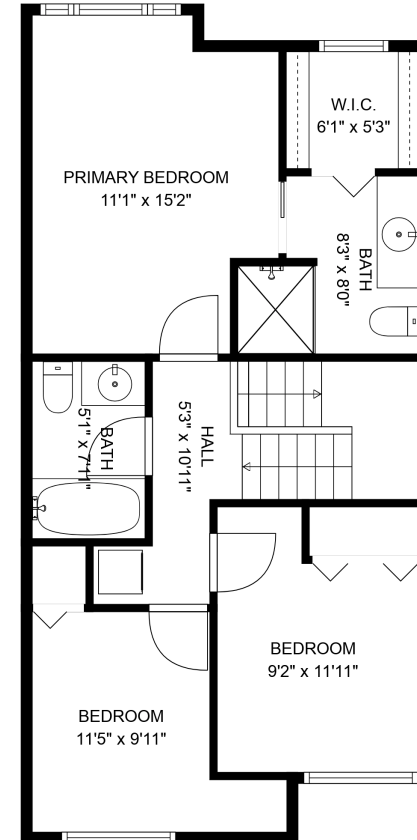
FLOOR 3
