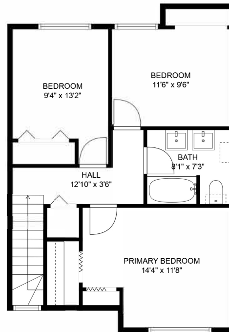
FLOOR 2
