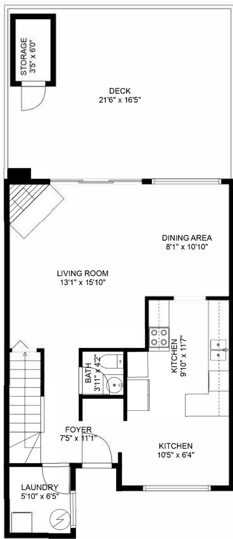
FLOOR 1
