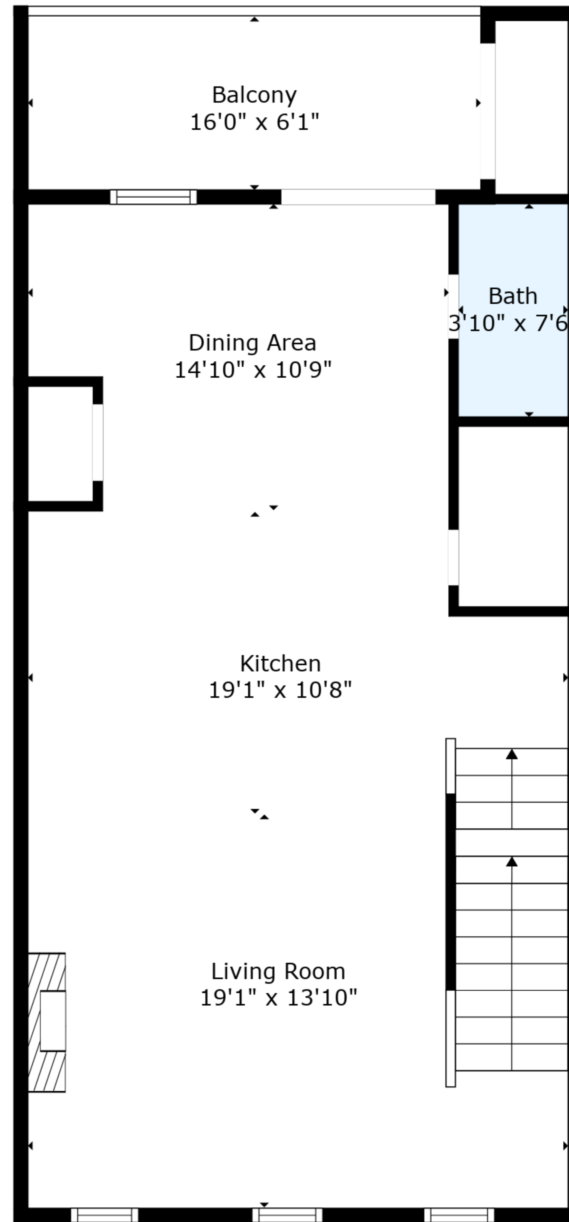
Floor 3
