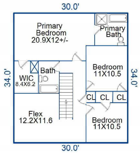
Second Floor 1020.0 sf
