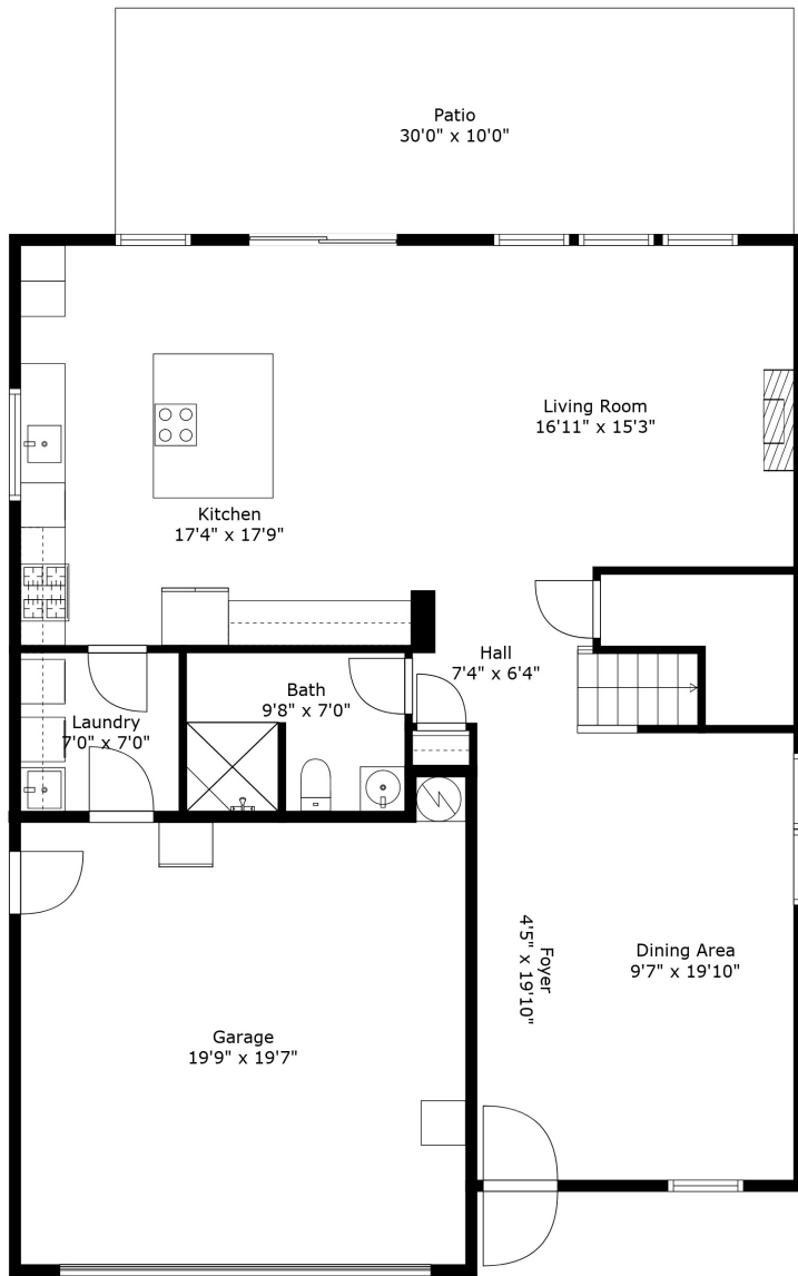
Floor 1
