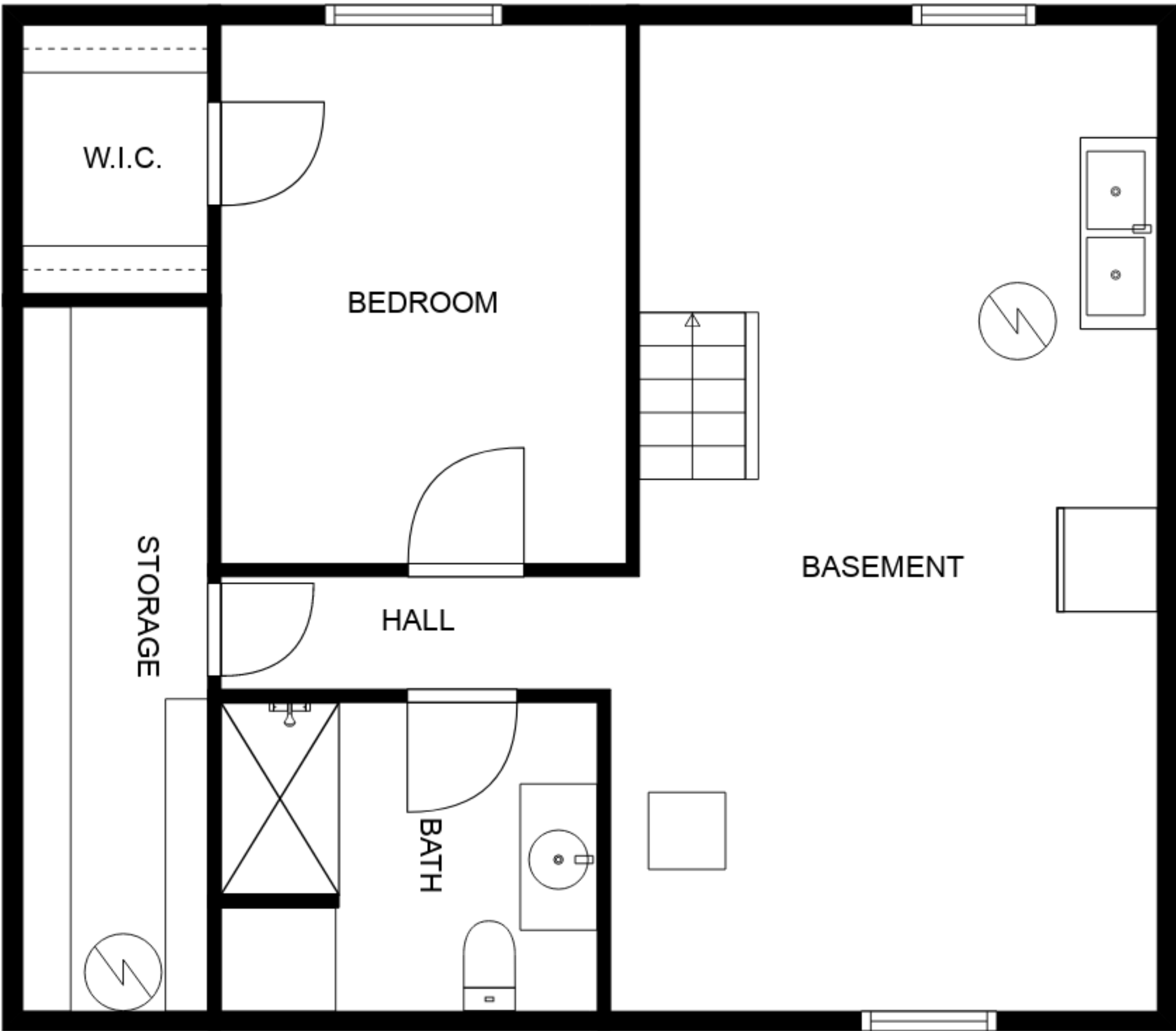
FLOOR 1
