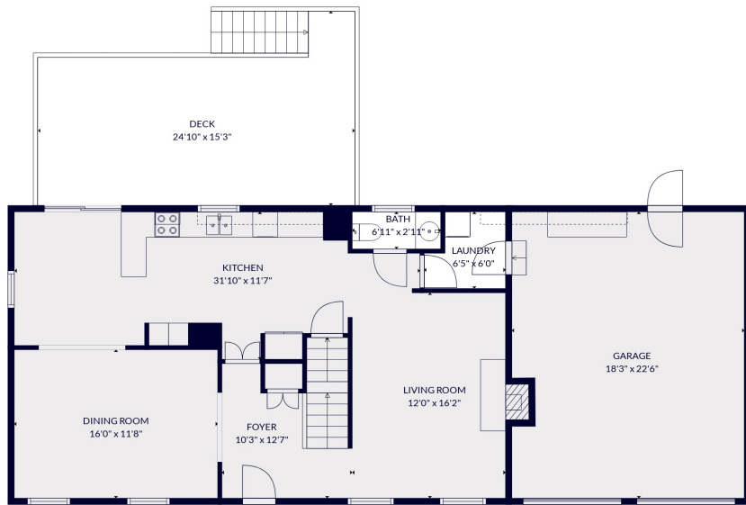
FLOOR 2
