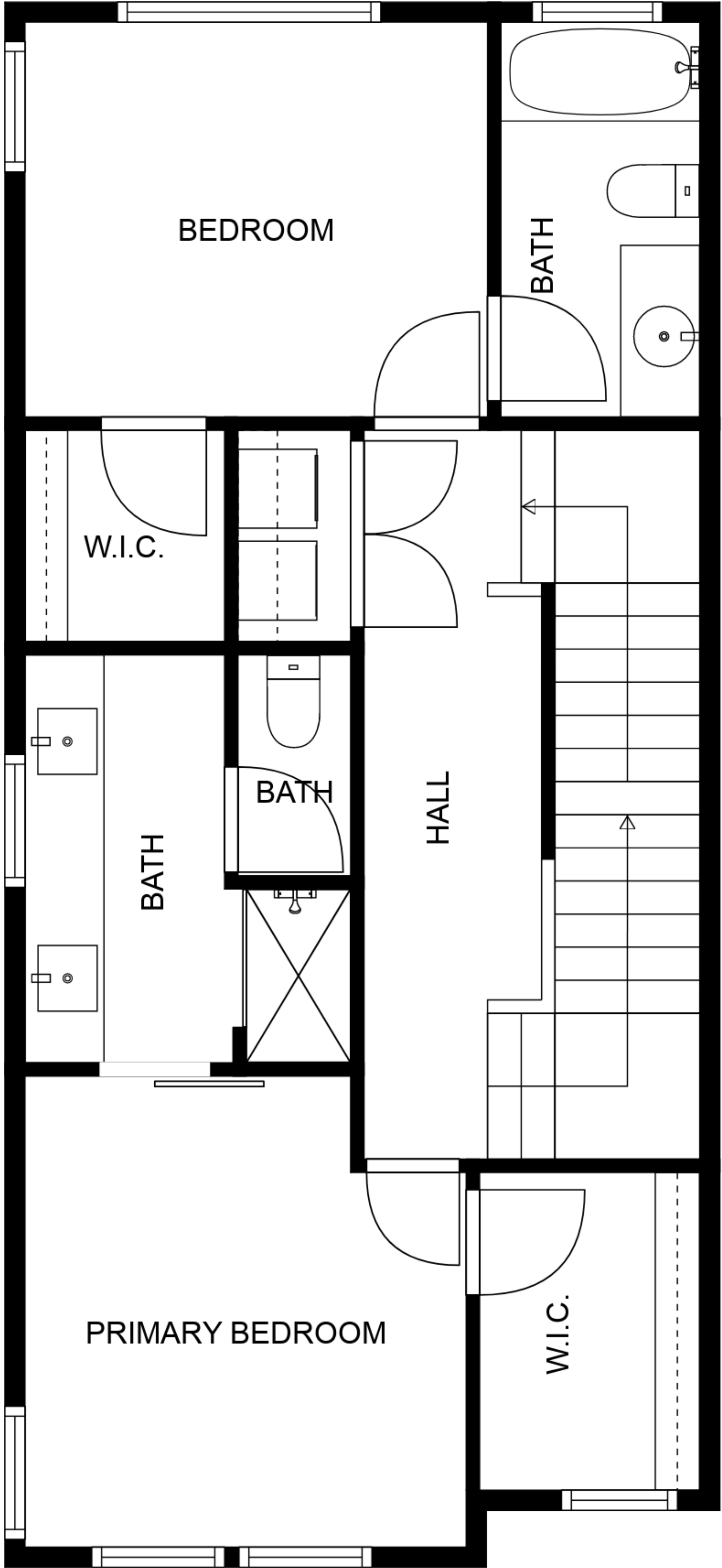
FLOOR 3
