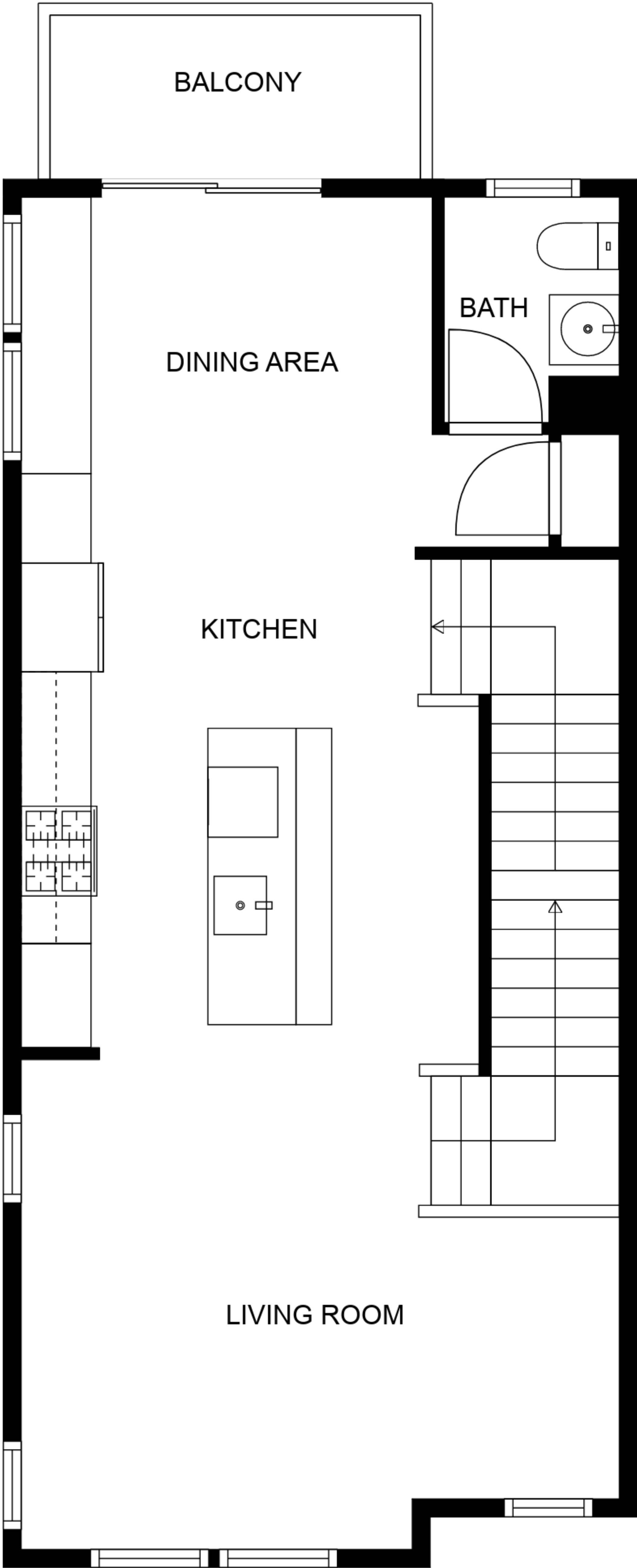
FLOOR 2
