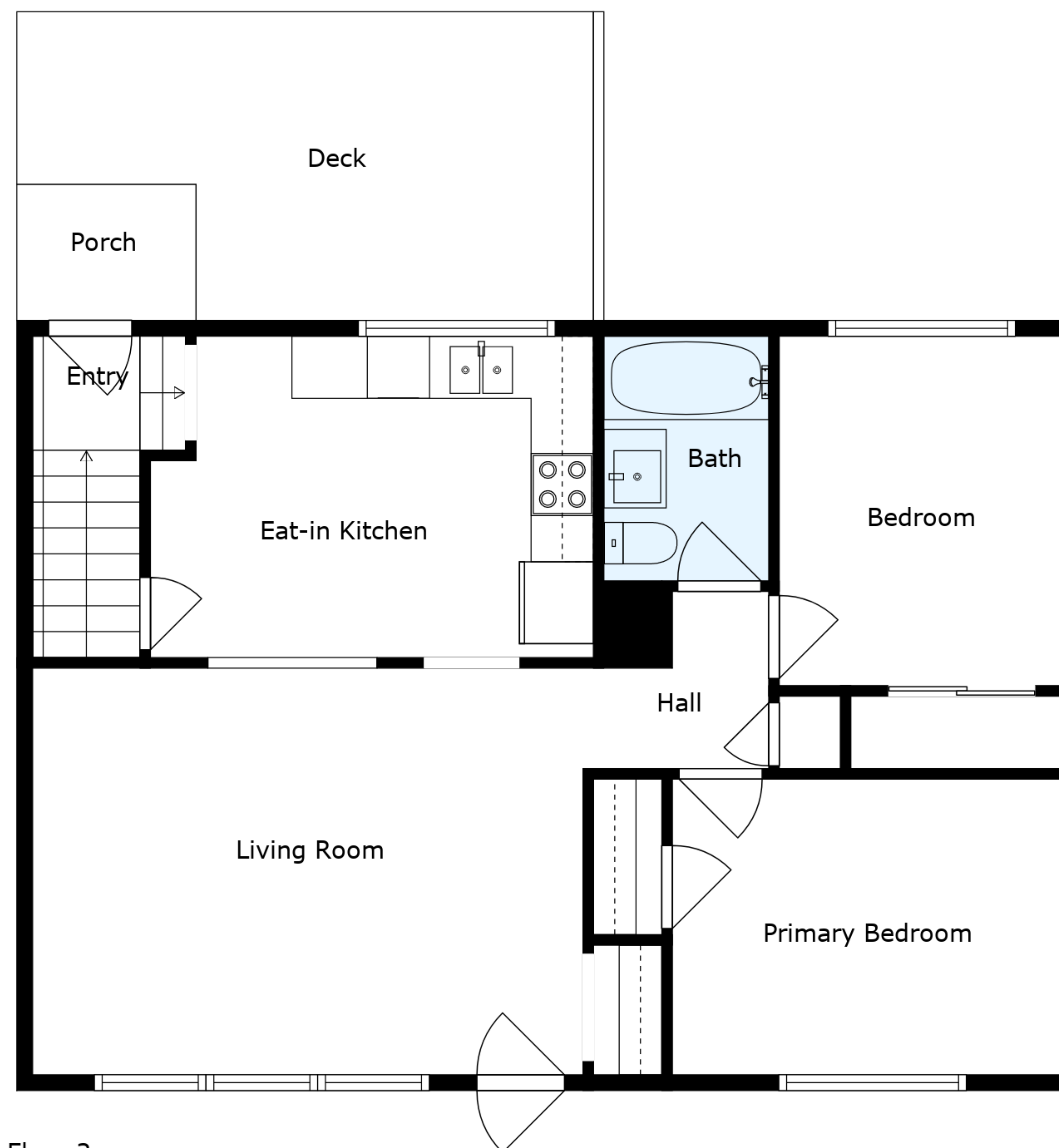
Floor 2
