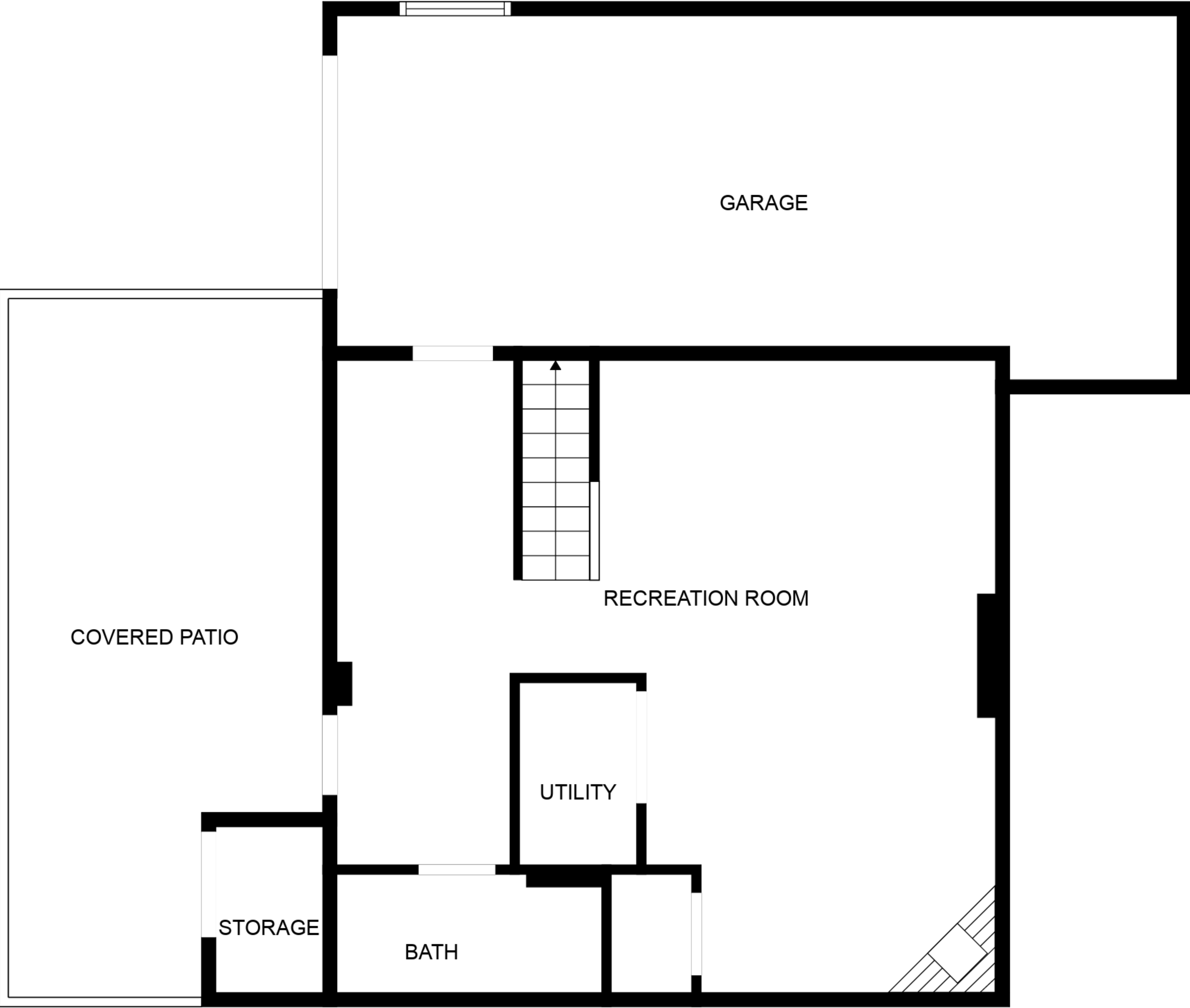
FLOOR 1
