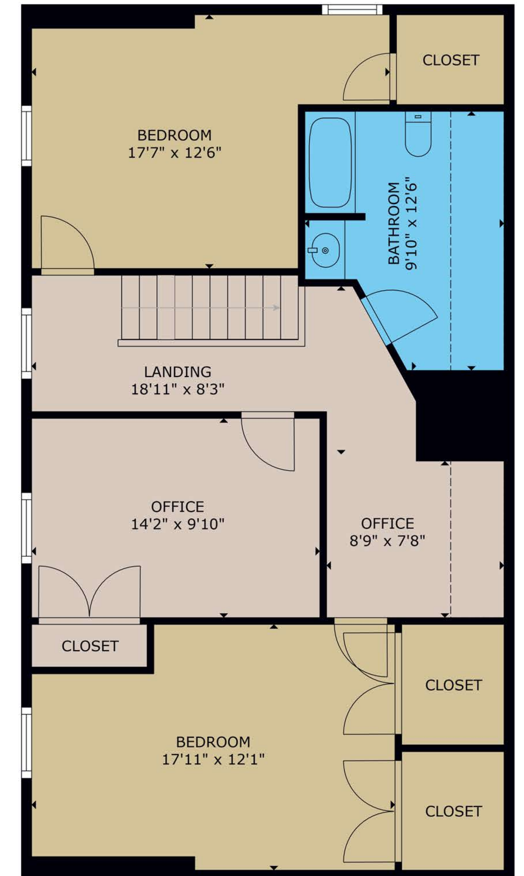
FLOOR 3
