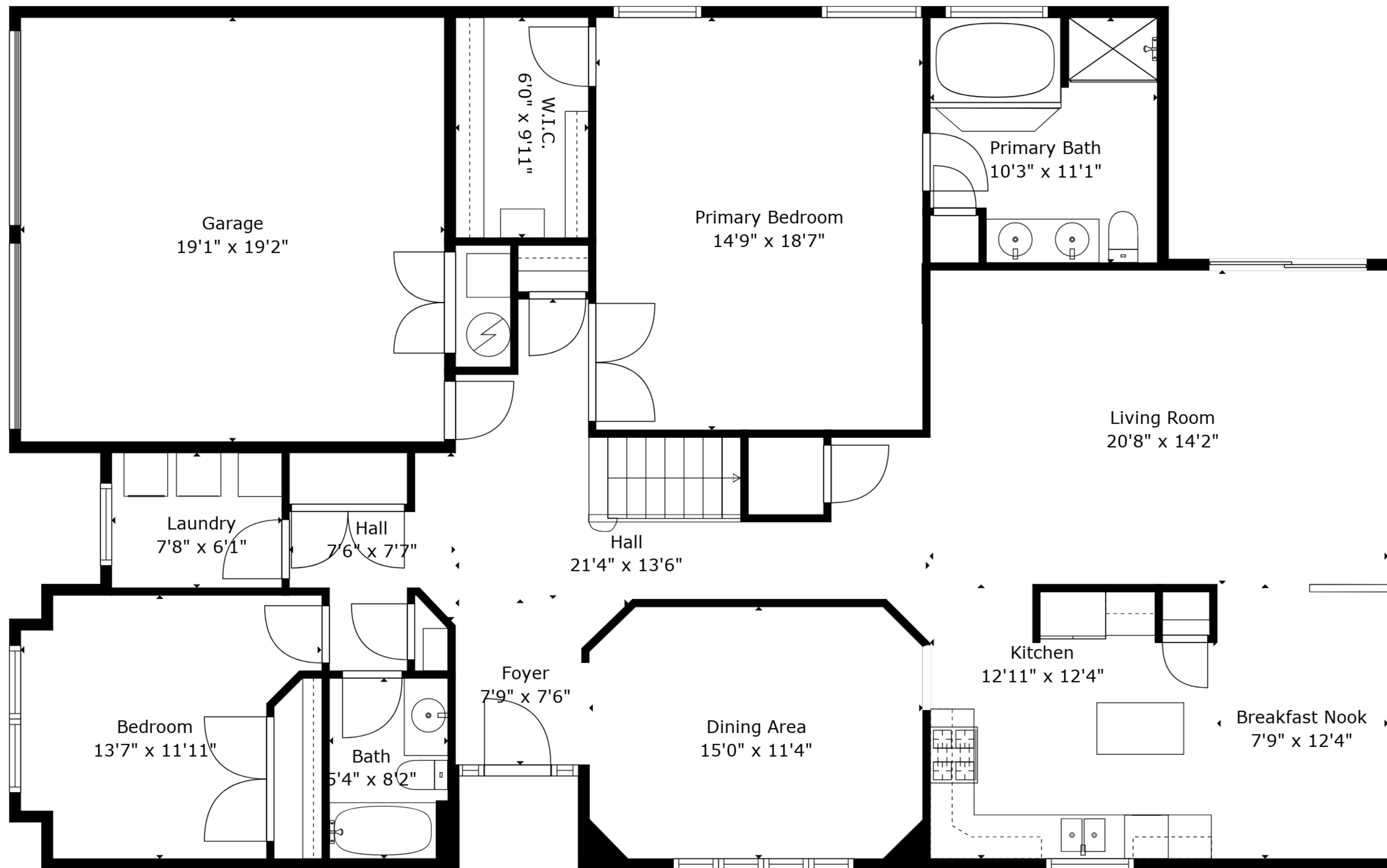
Floor 1
