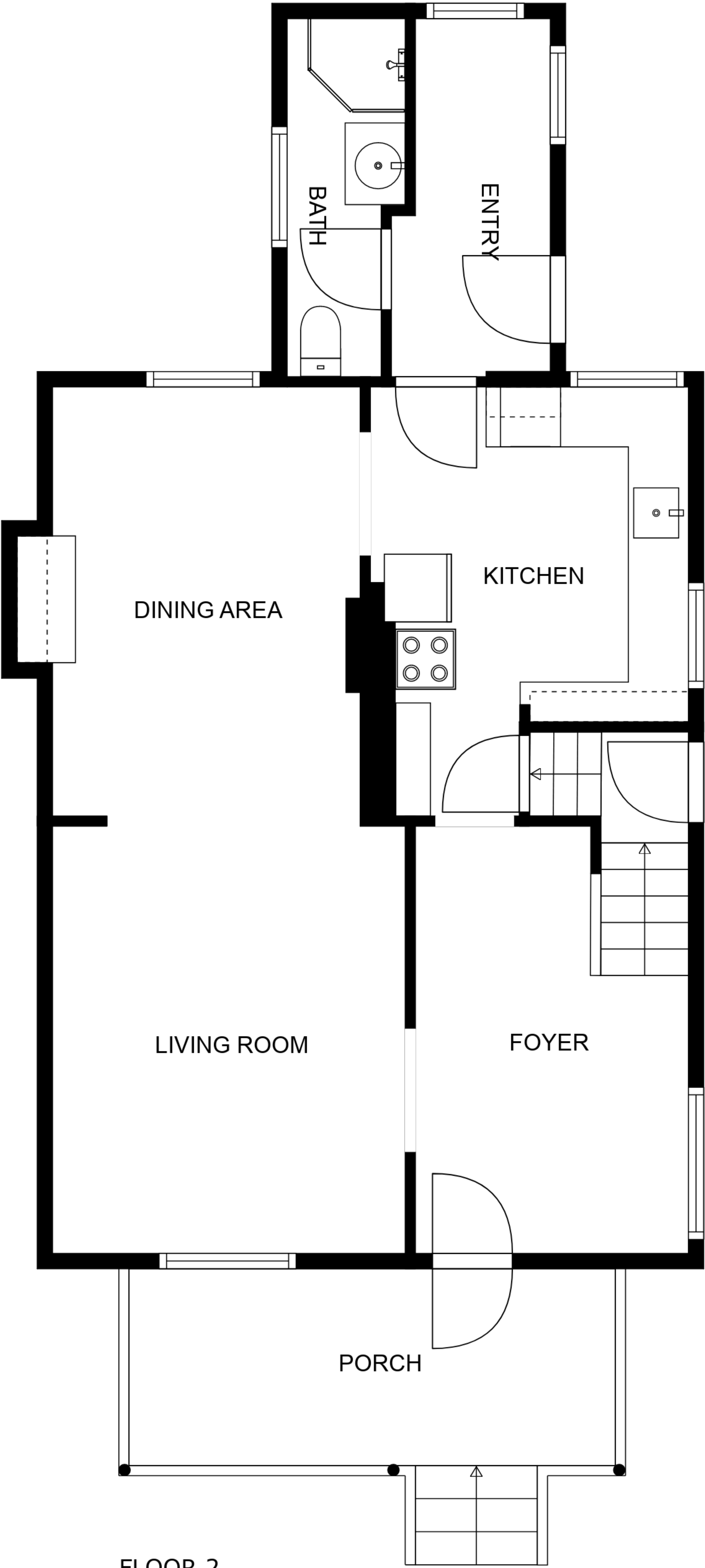
FLOOR 2
