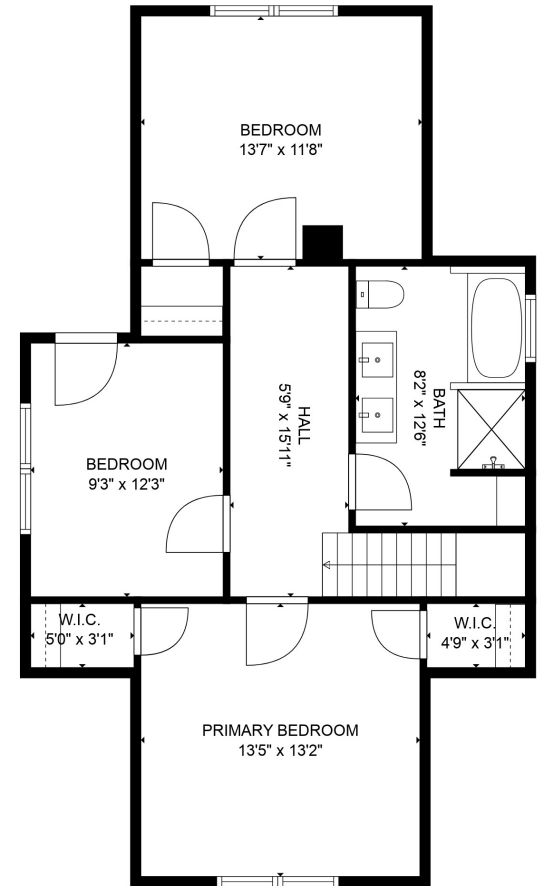
FLOOR 3
