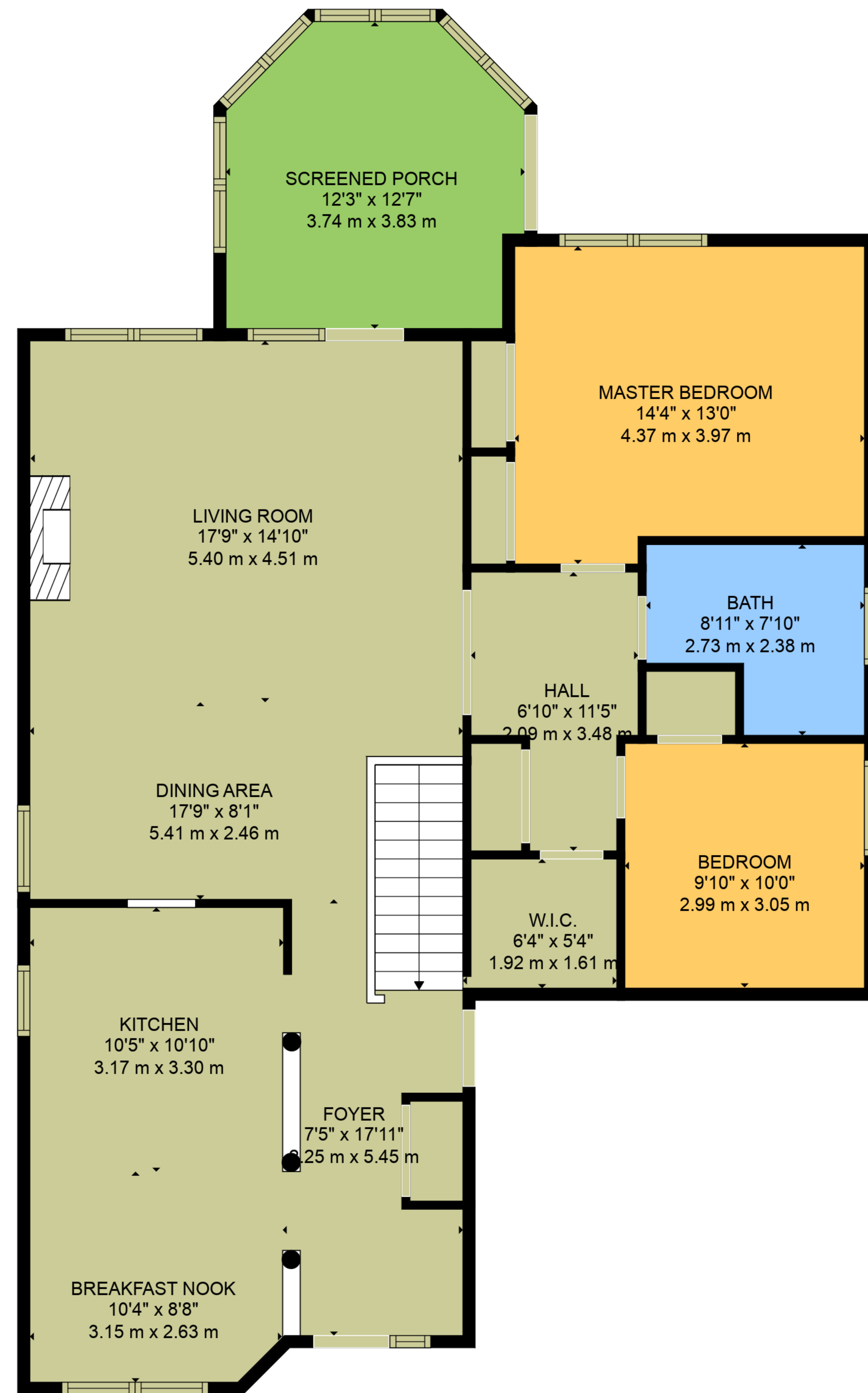
FLOOR 2
