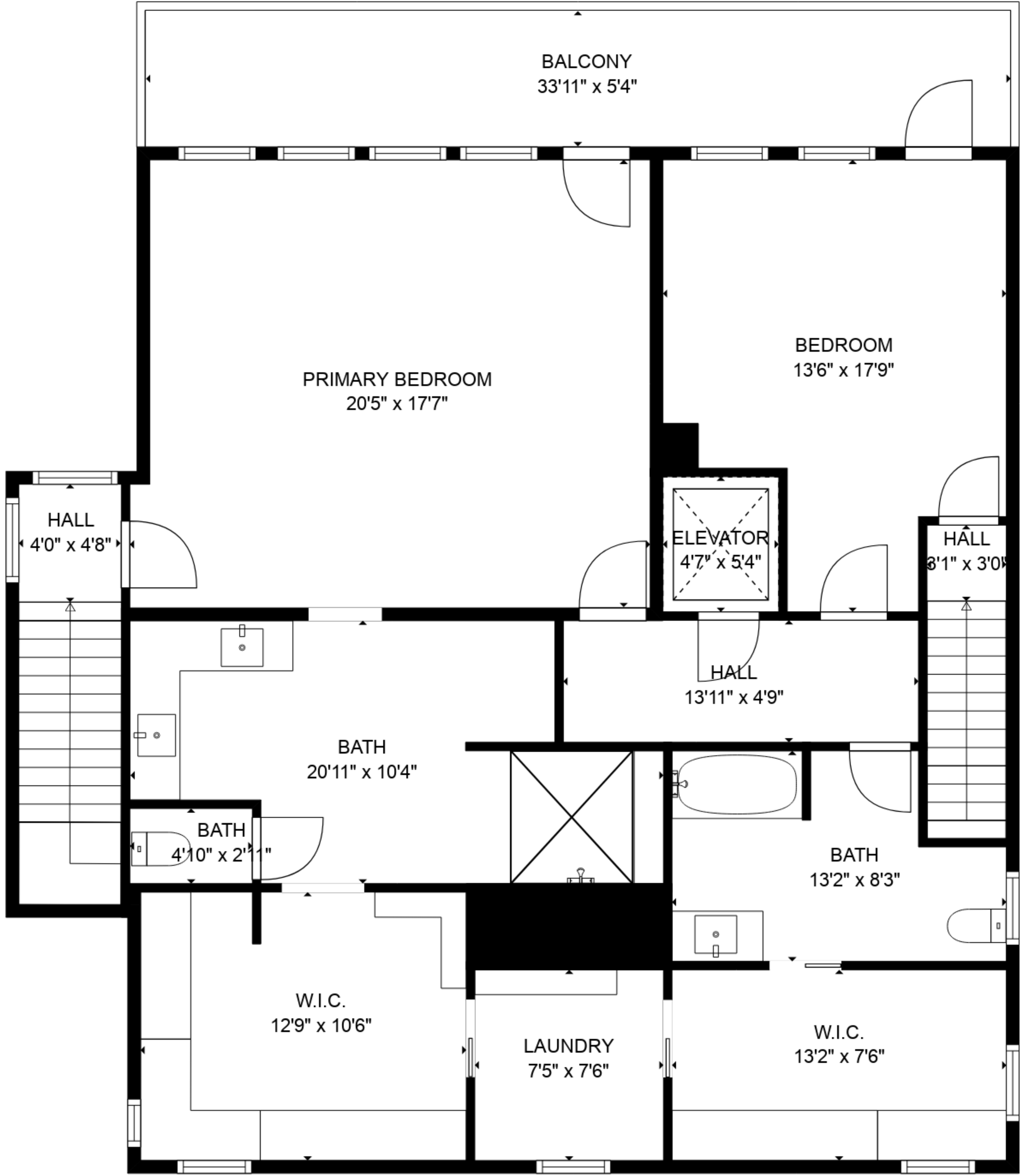
FLOOR 3
