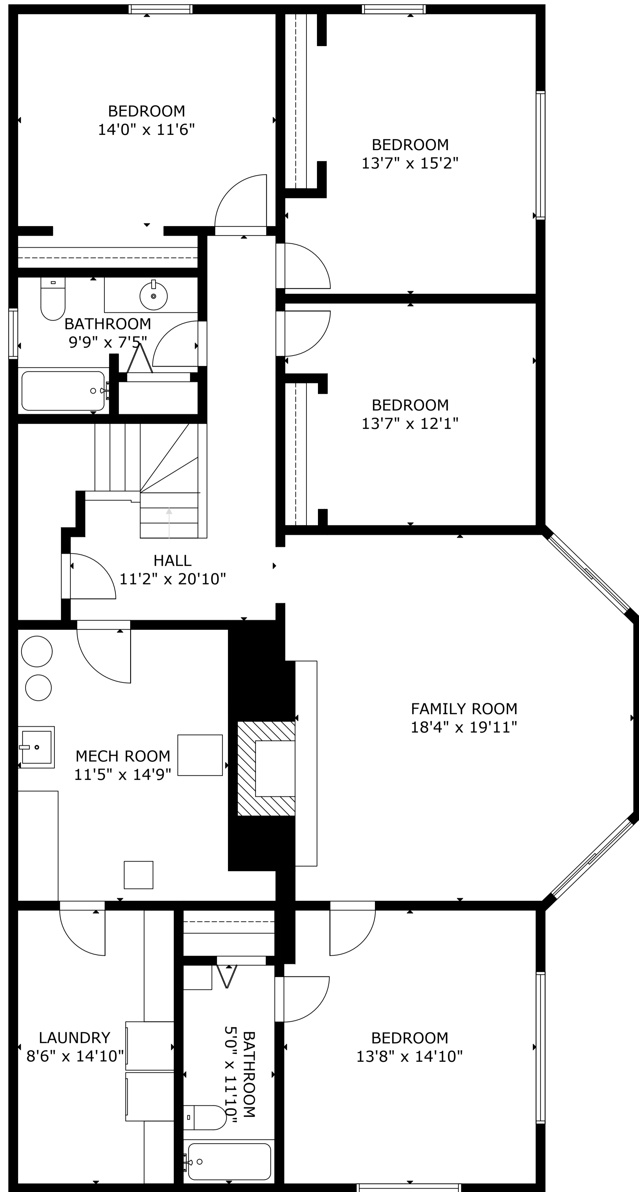
LOWER FLOOR
