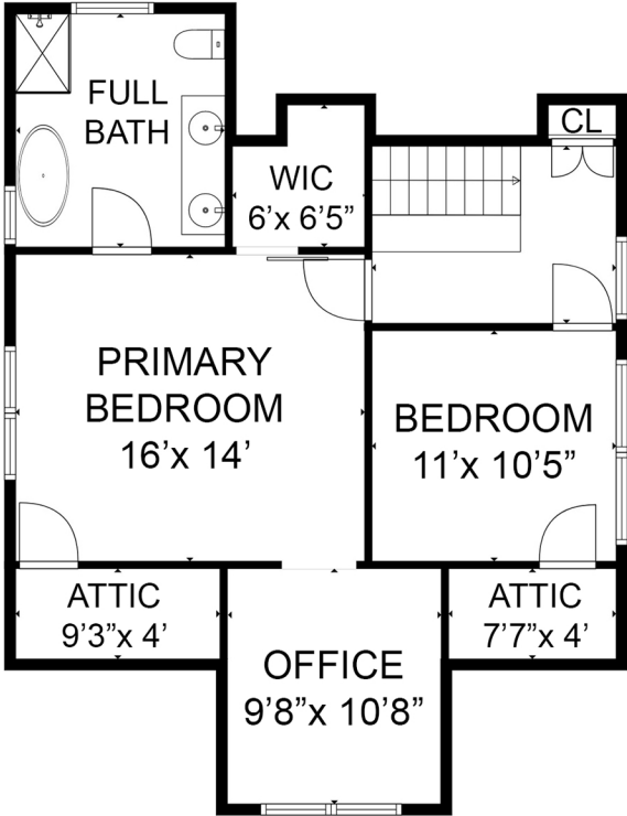
SECOND FLOOR
