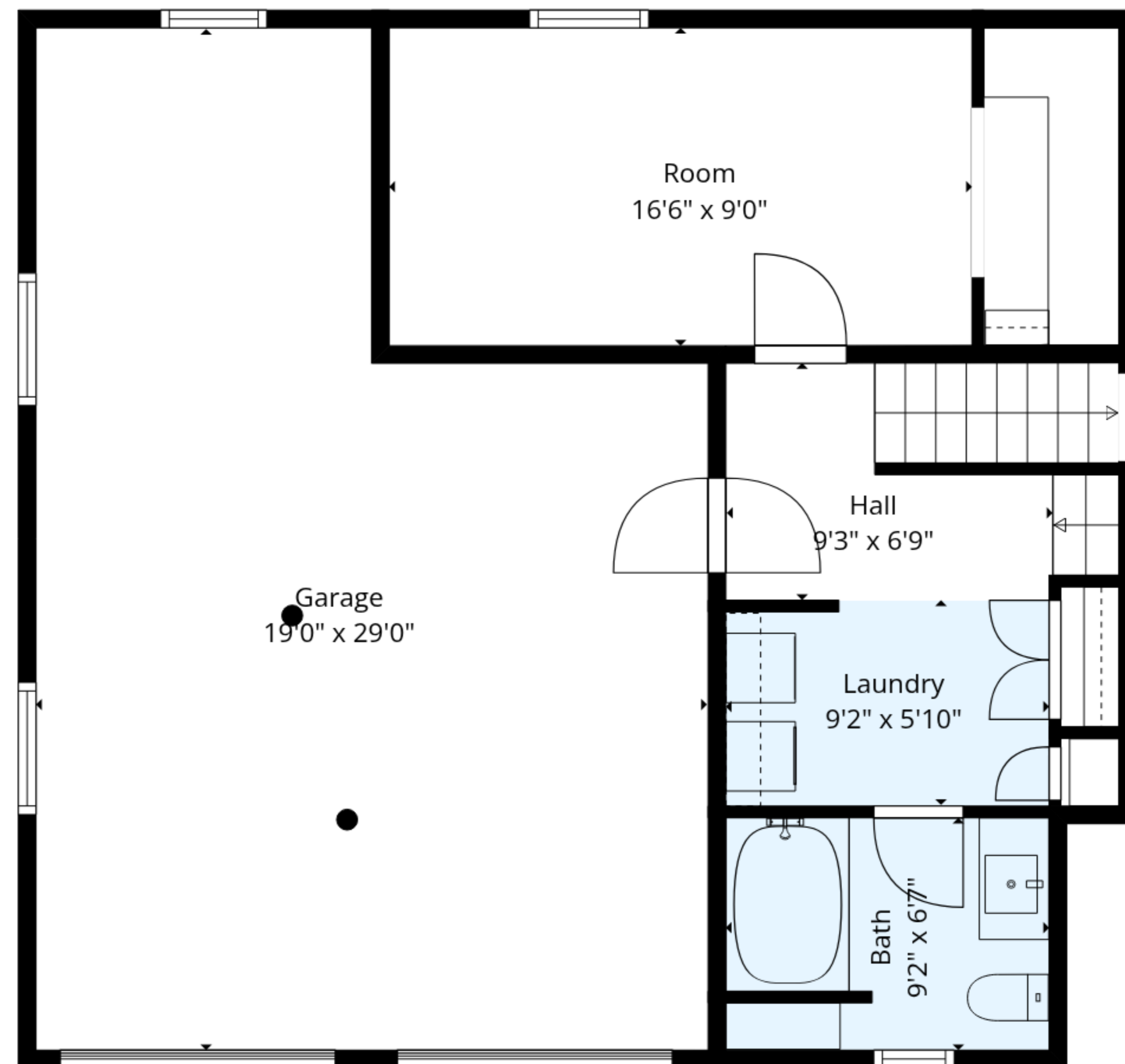
1st Floor
