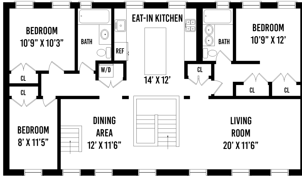
MAIN FLOOR
