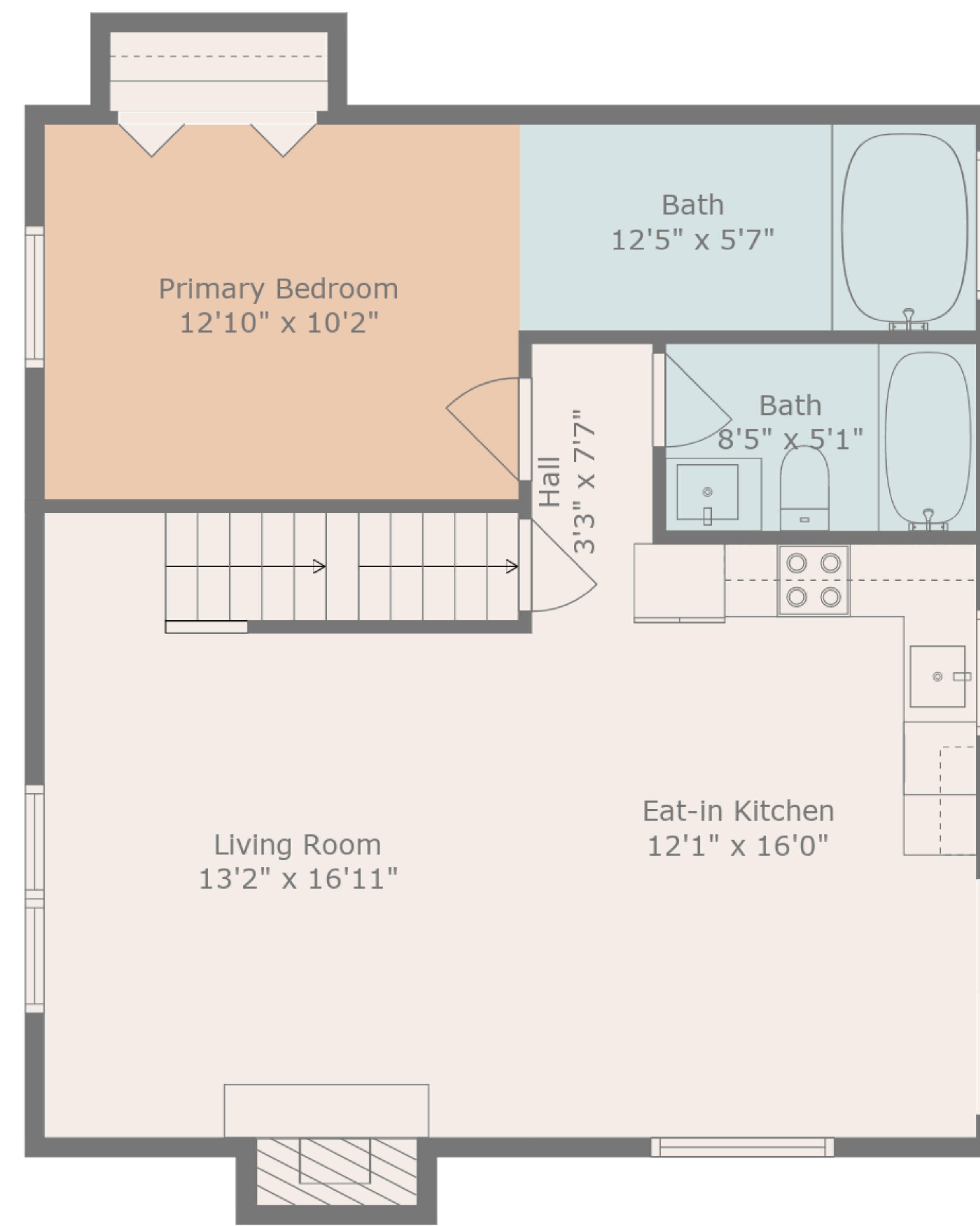
Floor 2
