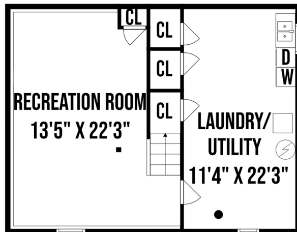
LOWER LEVEL
