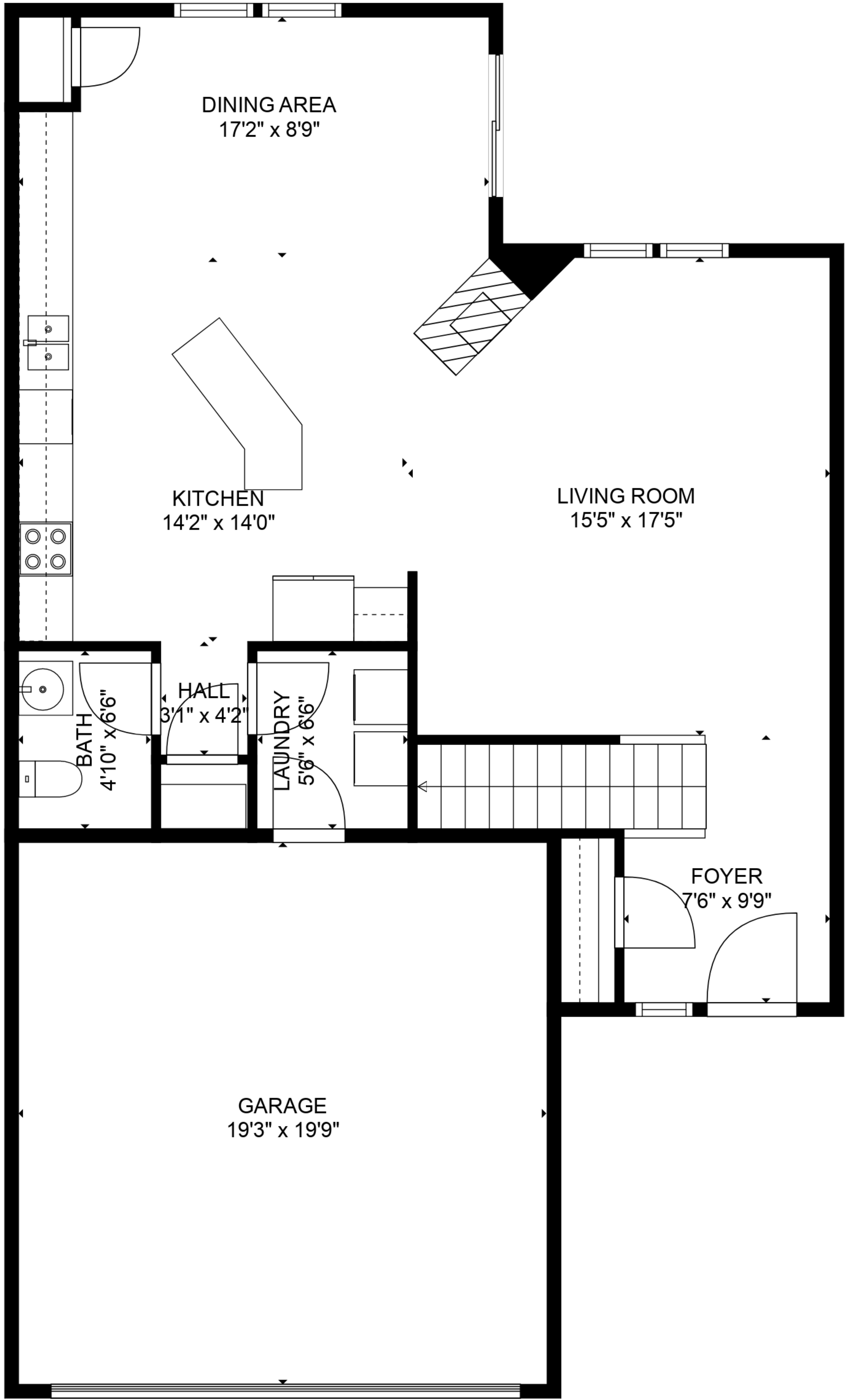
FLOOR 1
