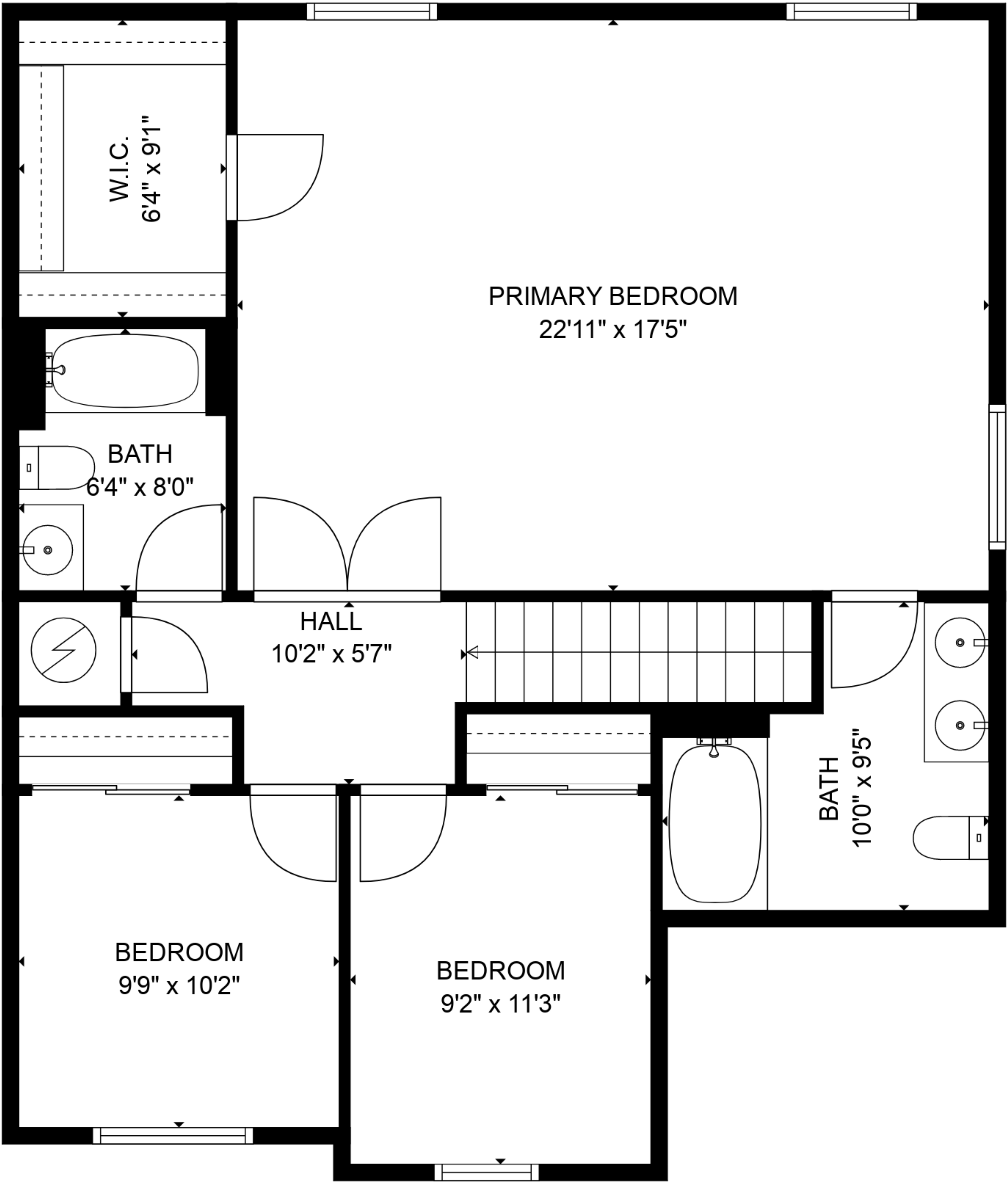
FLOOR 2
