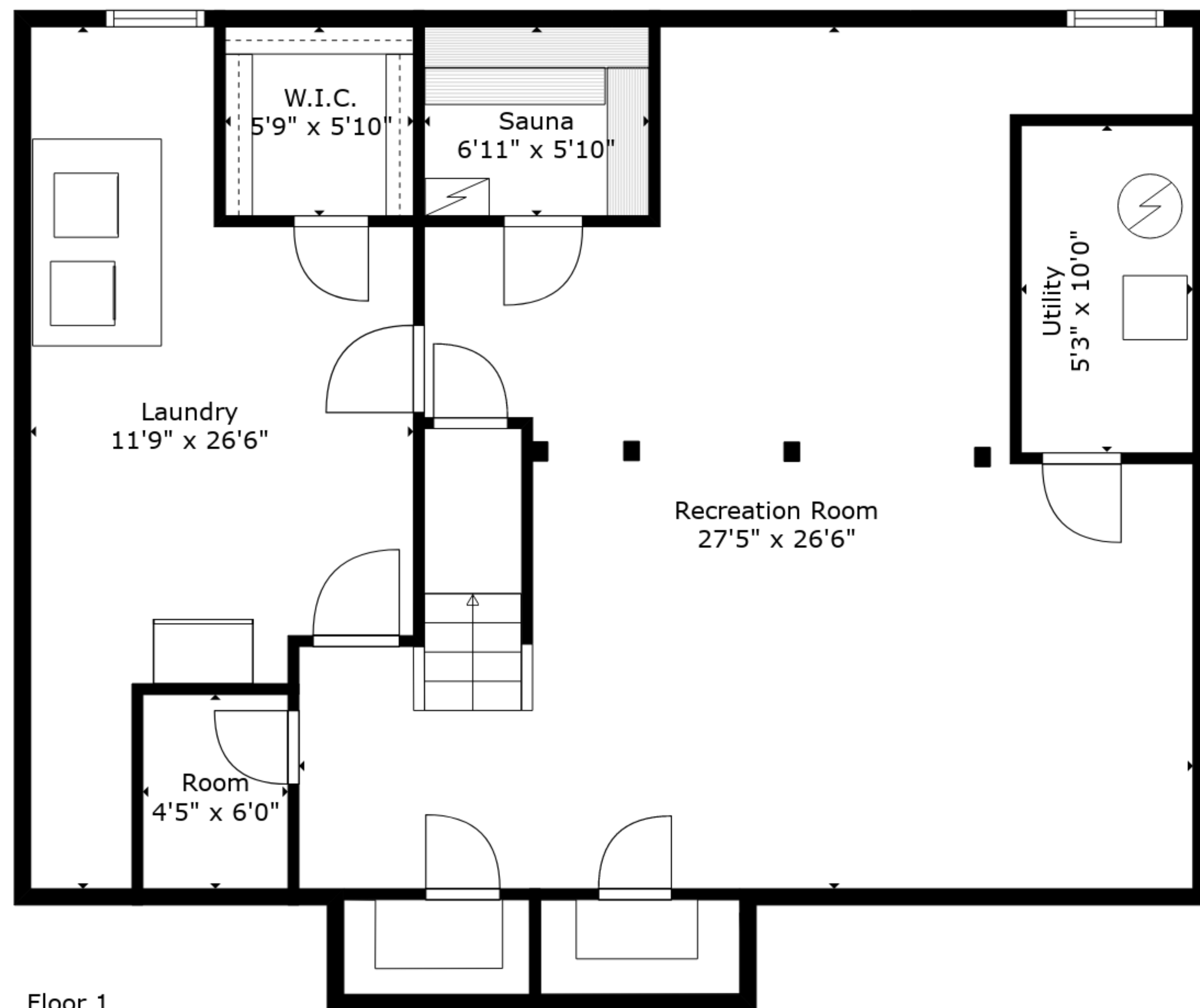
Floor 1
