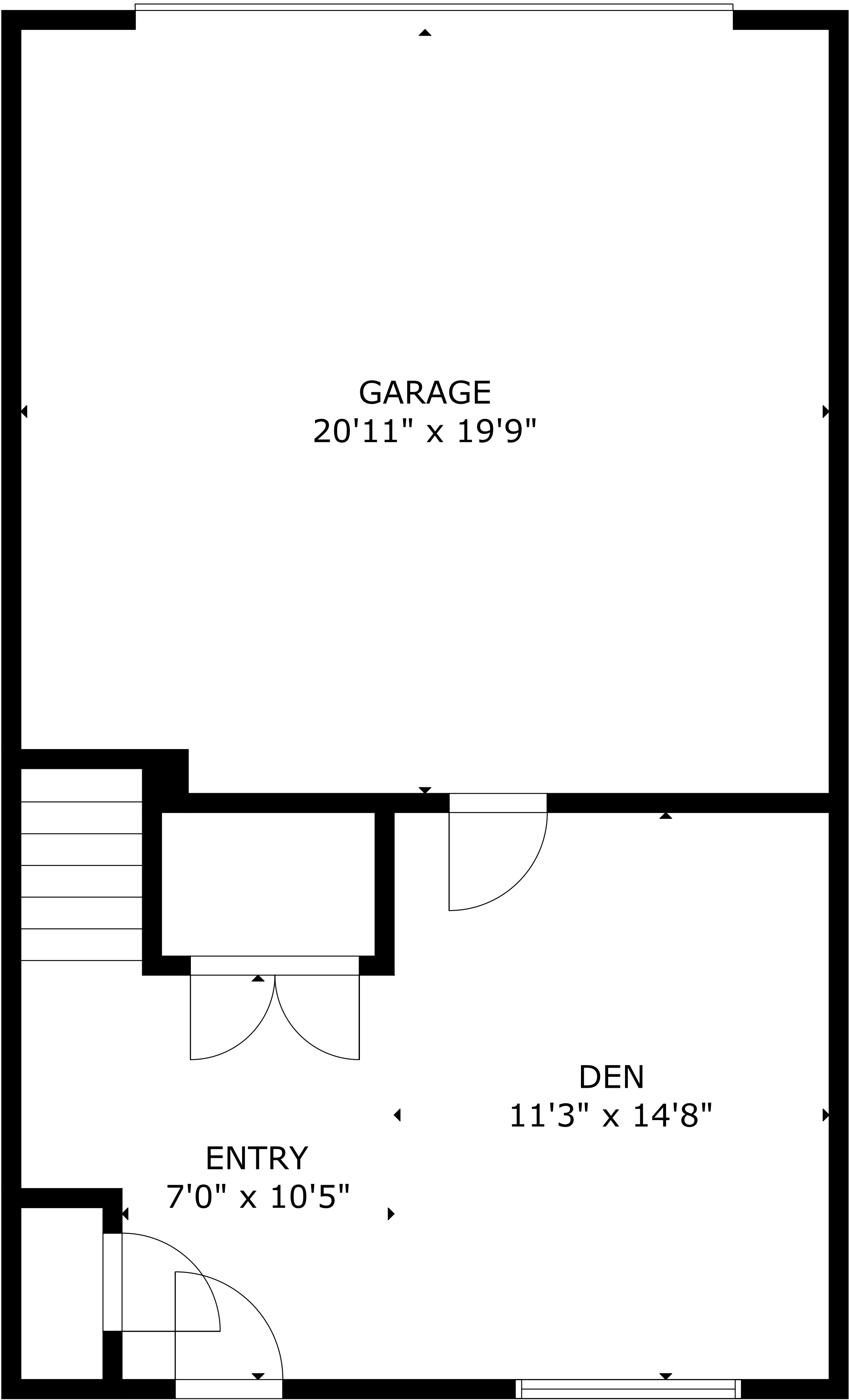
LOWER FLOOR
