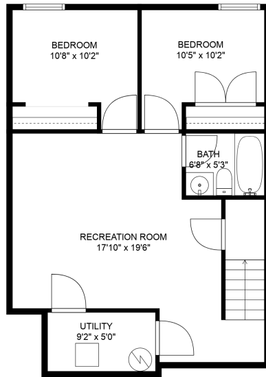
FLOOR 1
