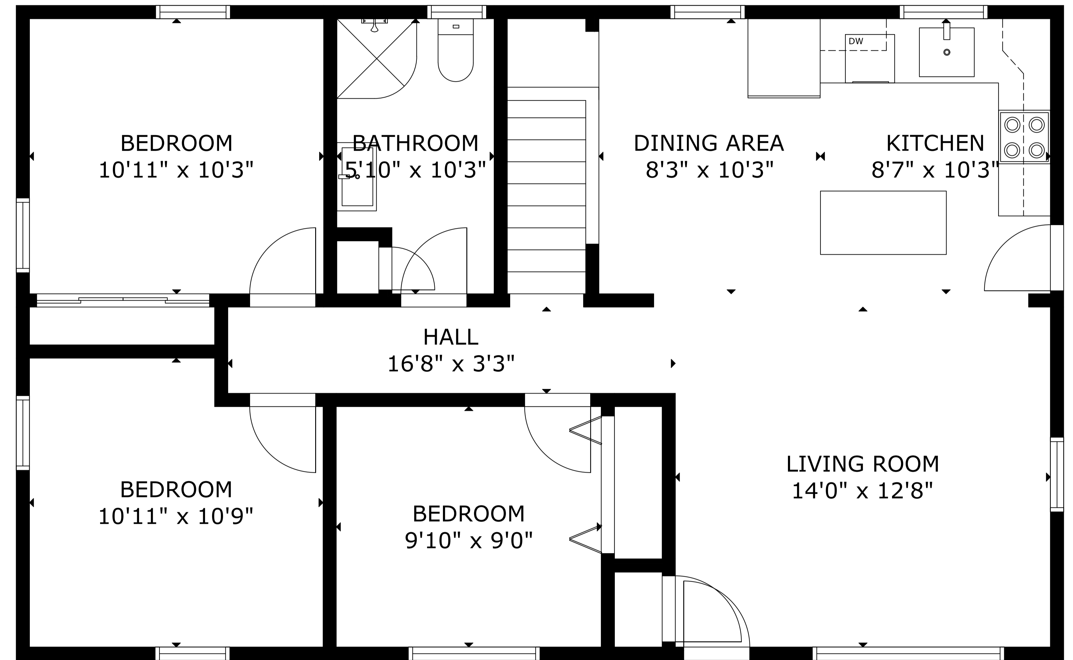
MAIN FLOOR
