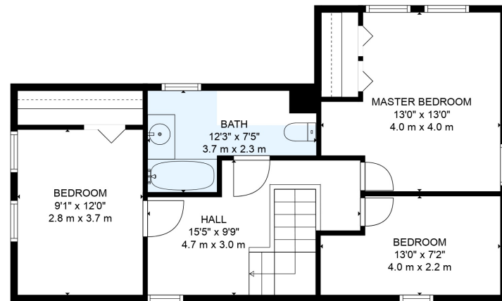
FLOOR 3
