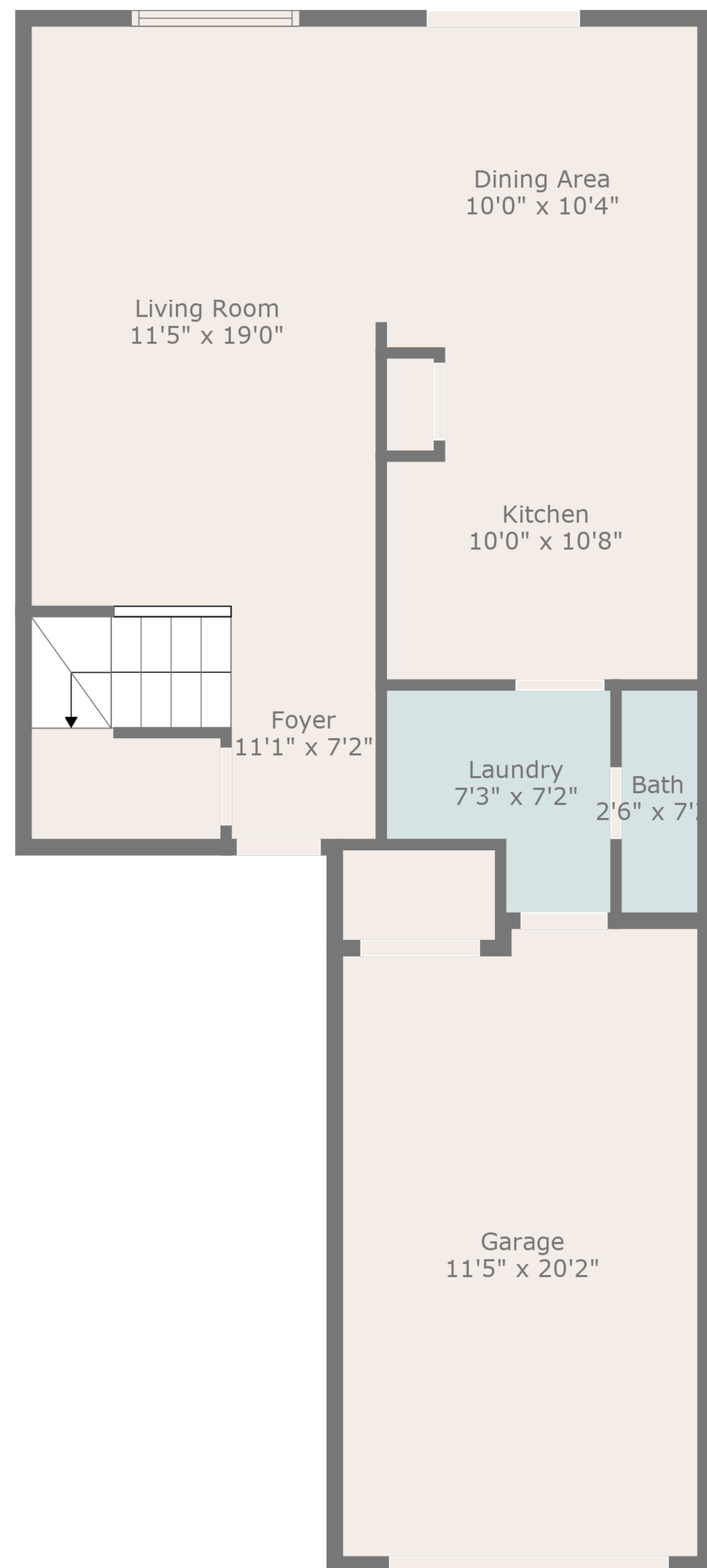
Floor 1
