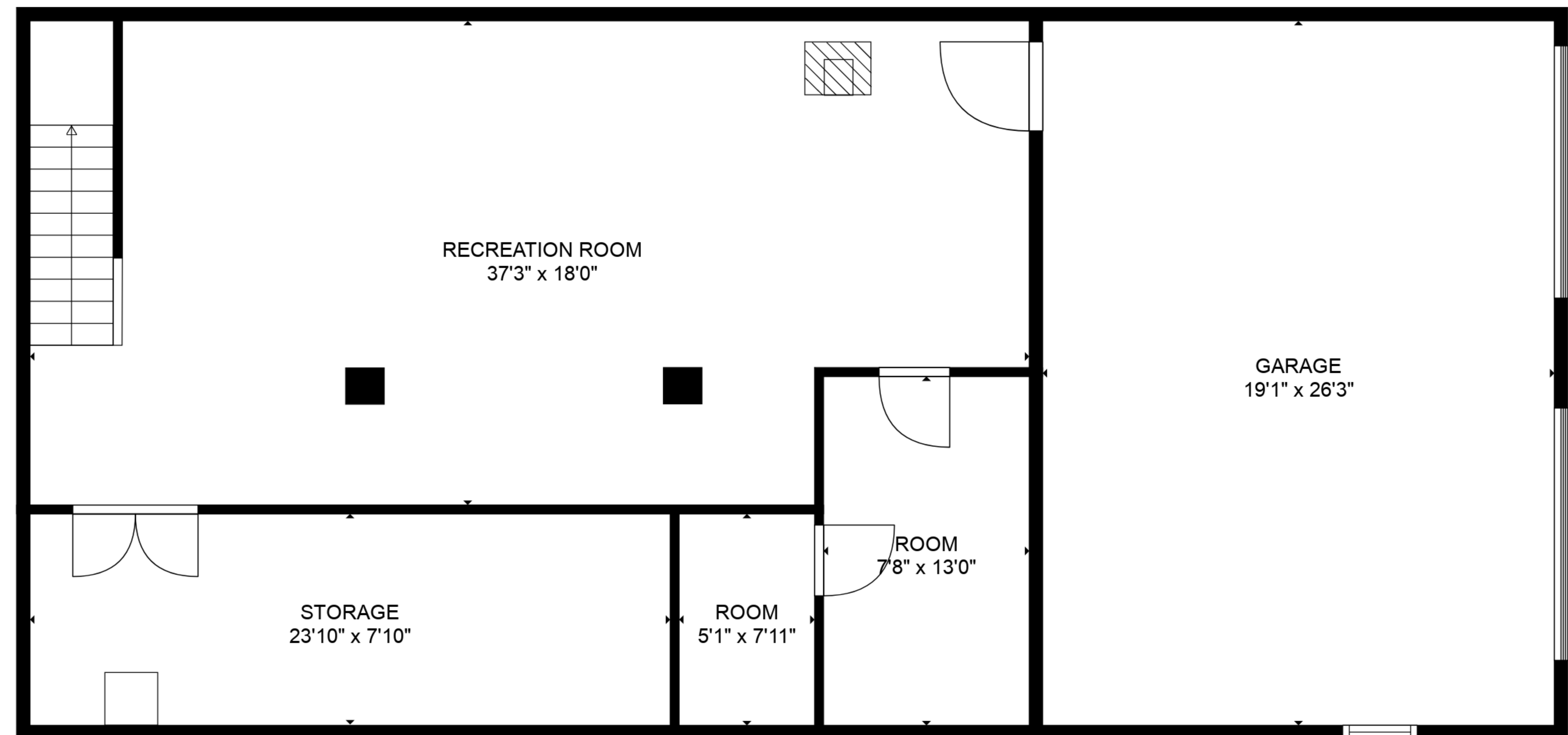
FLOOR 2
