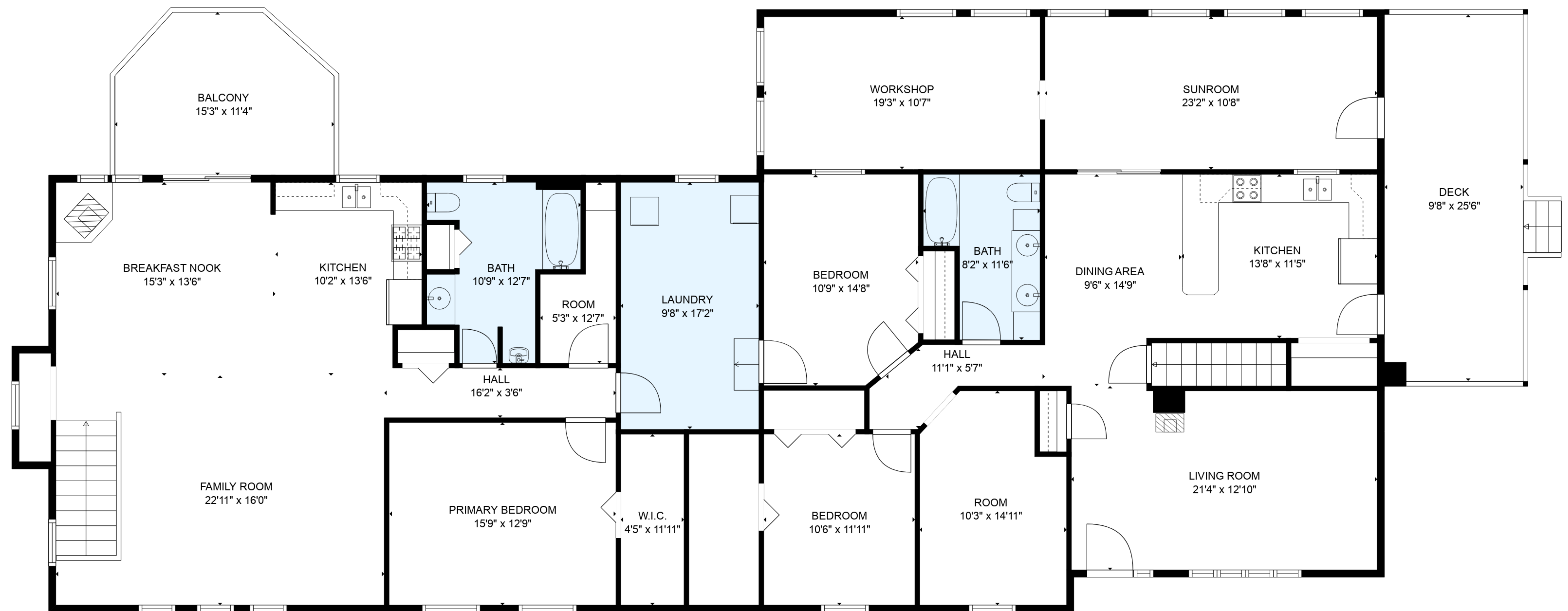
FLOOR 2
