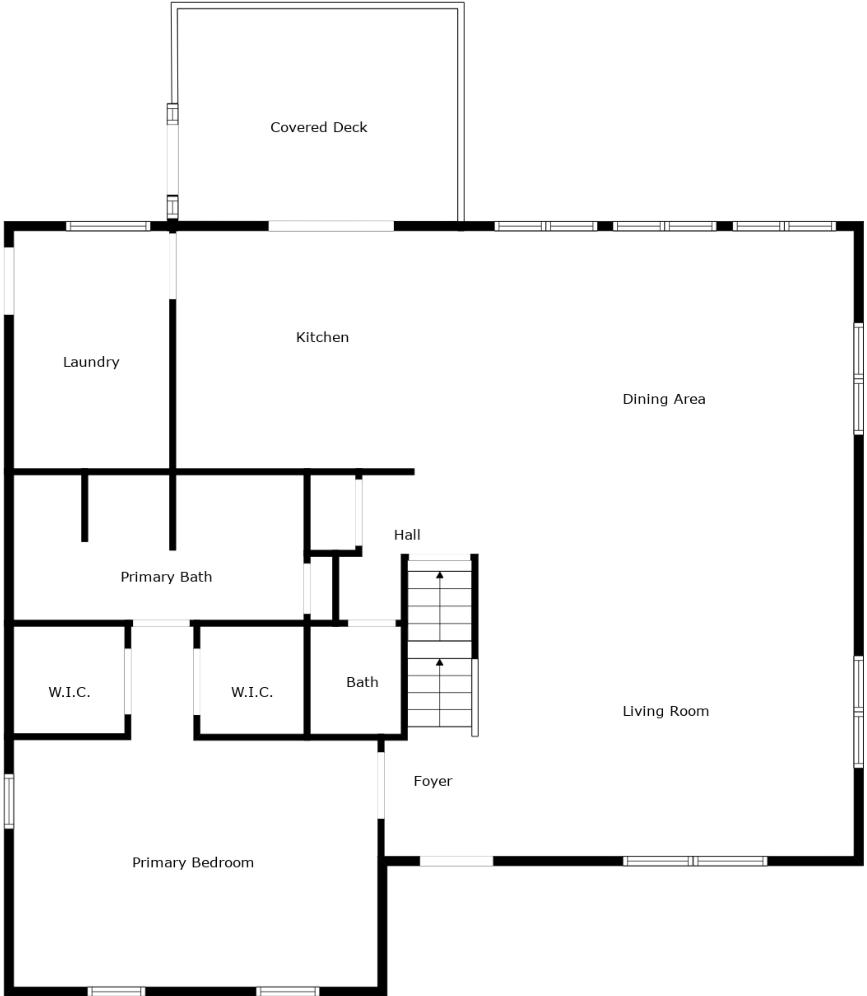
Floor 2
