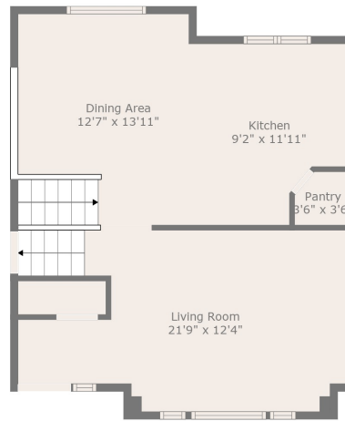
Floor 3
