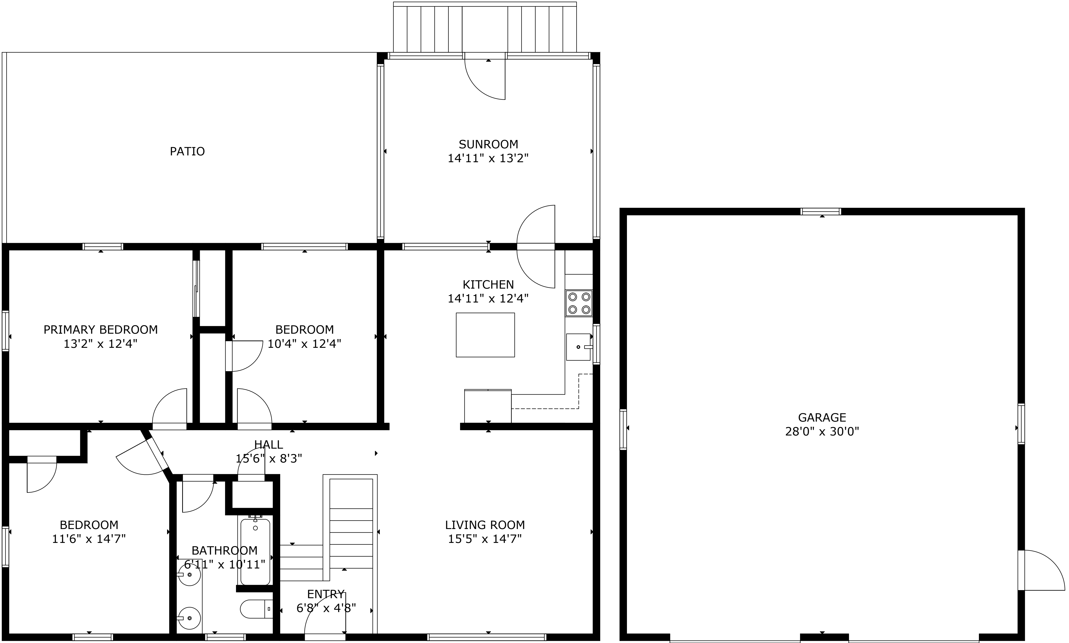
MAIN FLOOR
