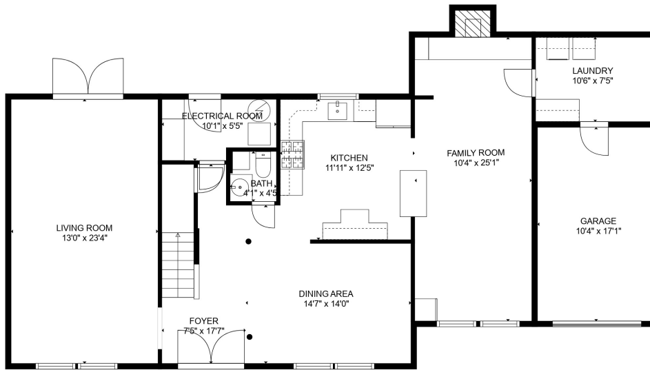
FLOOR 1
