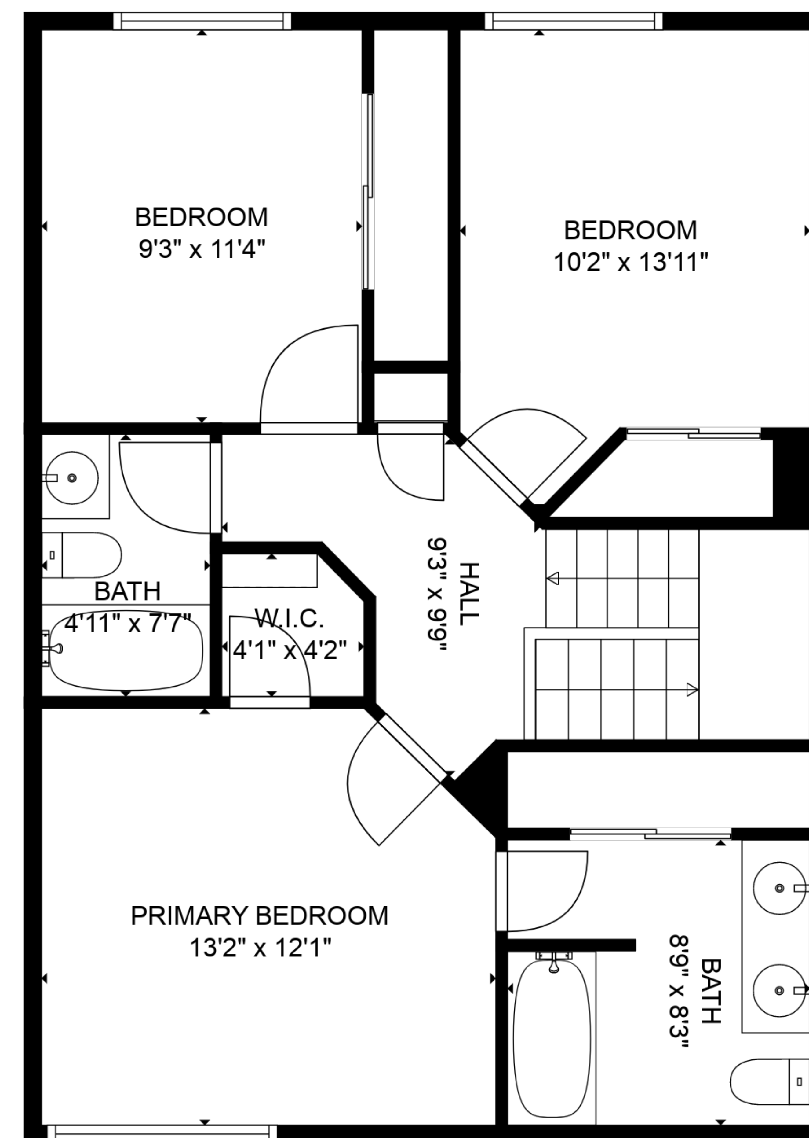
FLOOR 2
