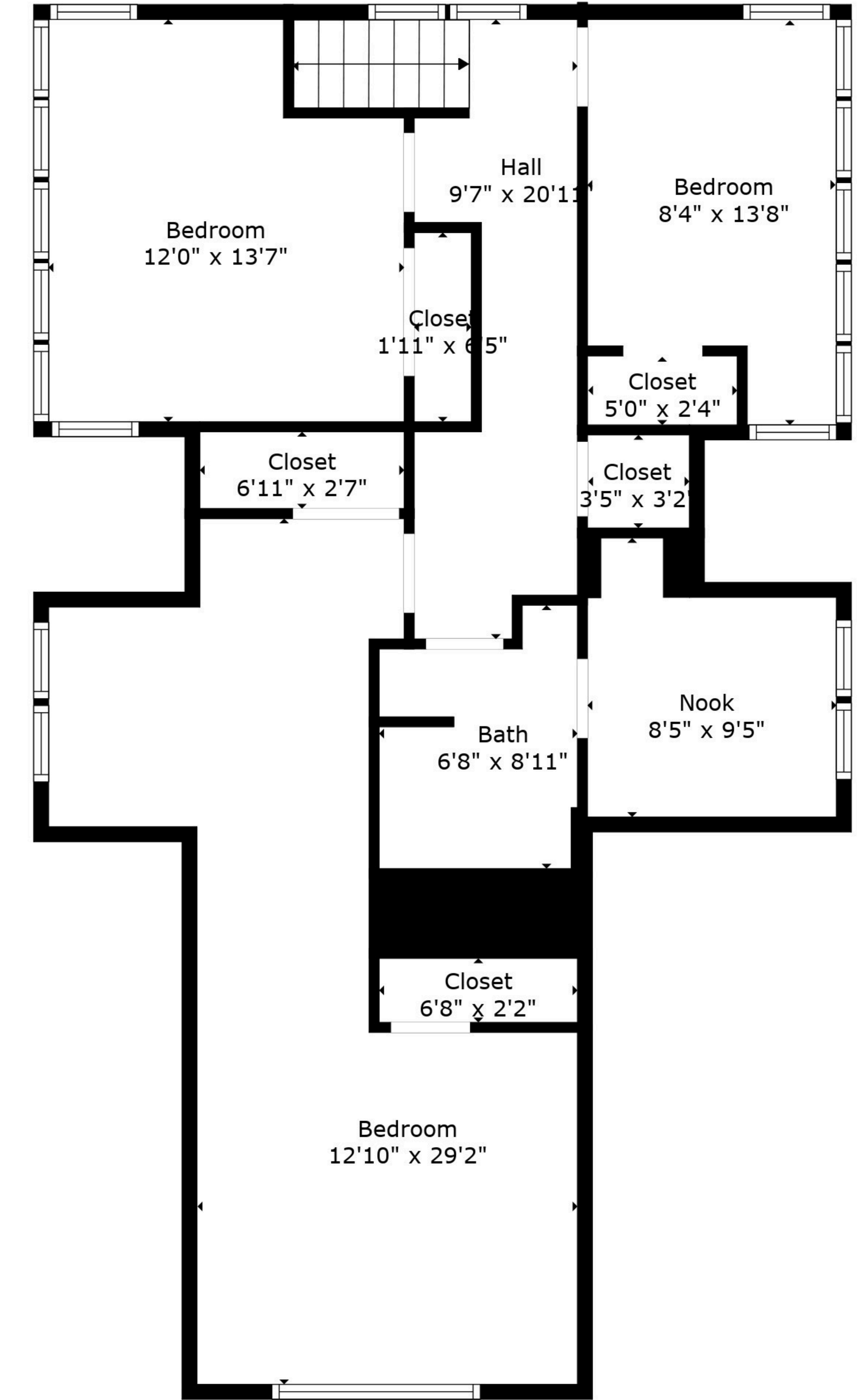
Floor 2
