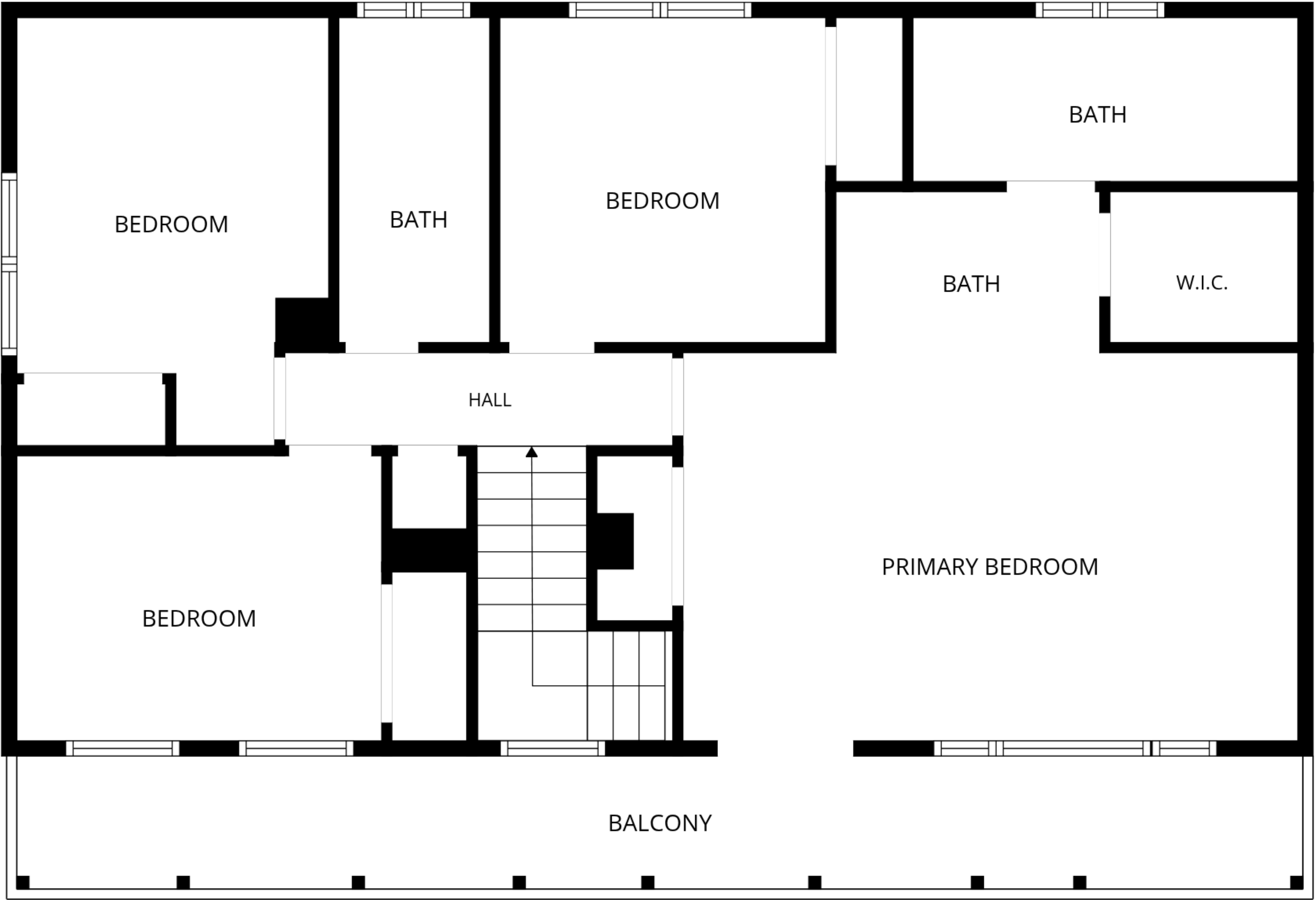
2nd floor
