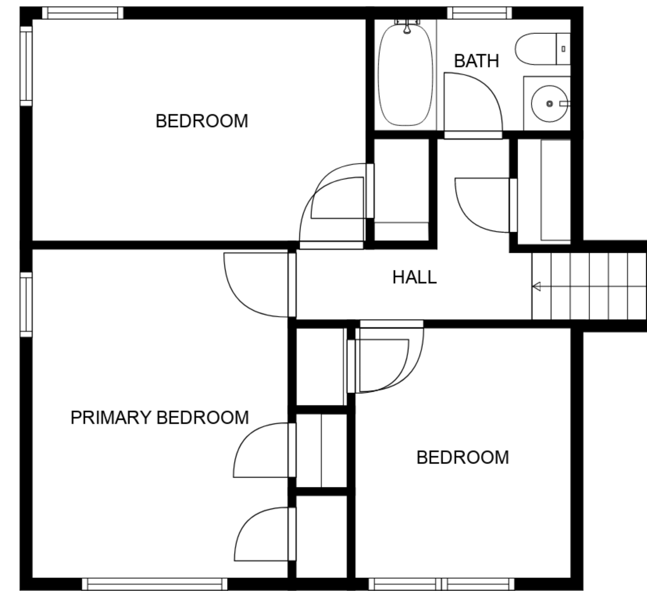
FLOOR 4
