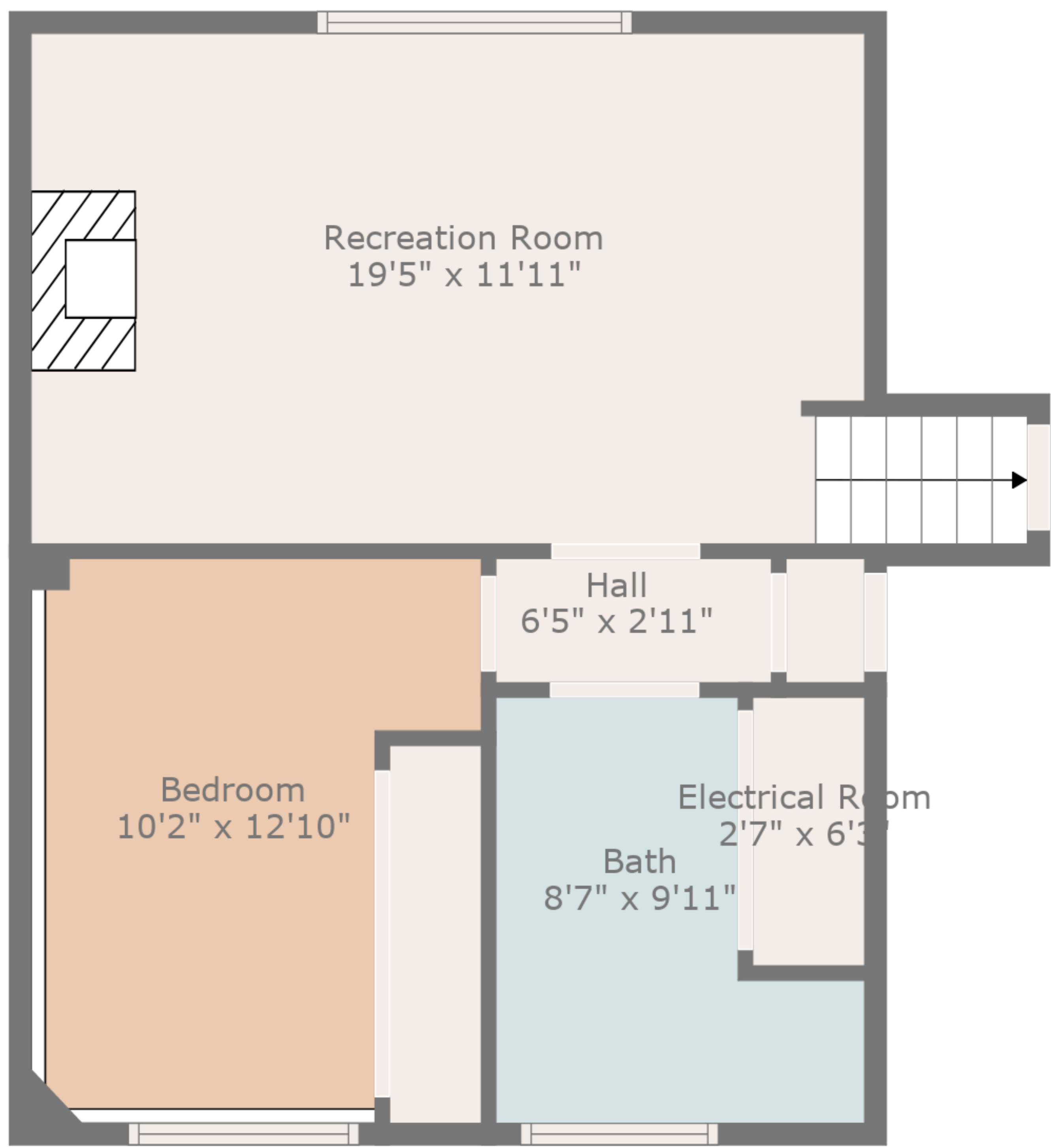
Floor 1
