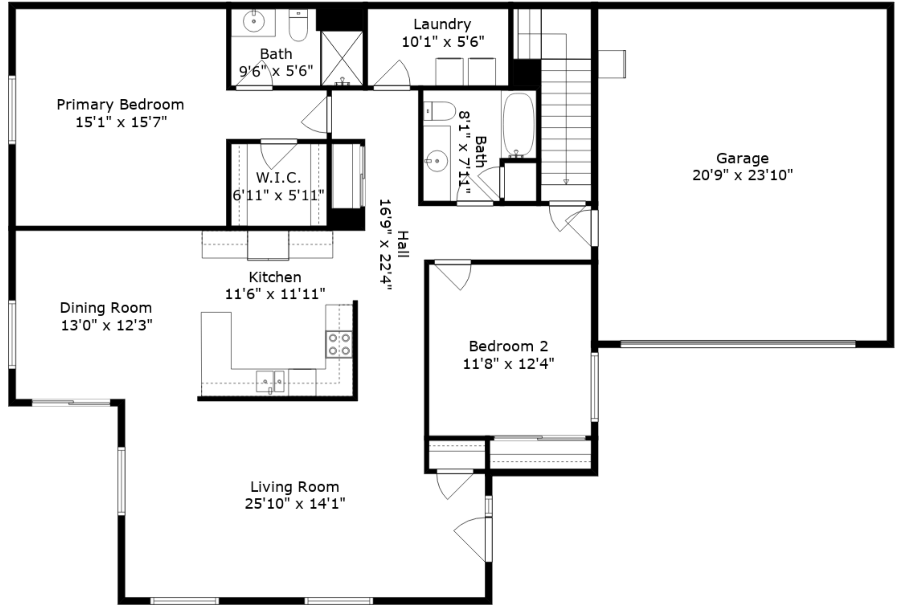
Main Floor
