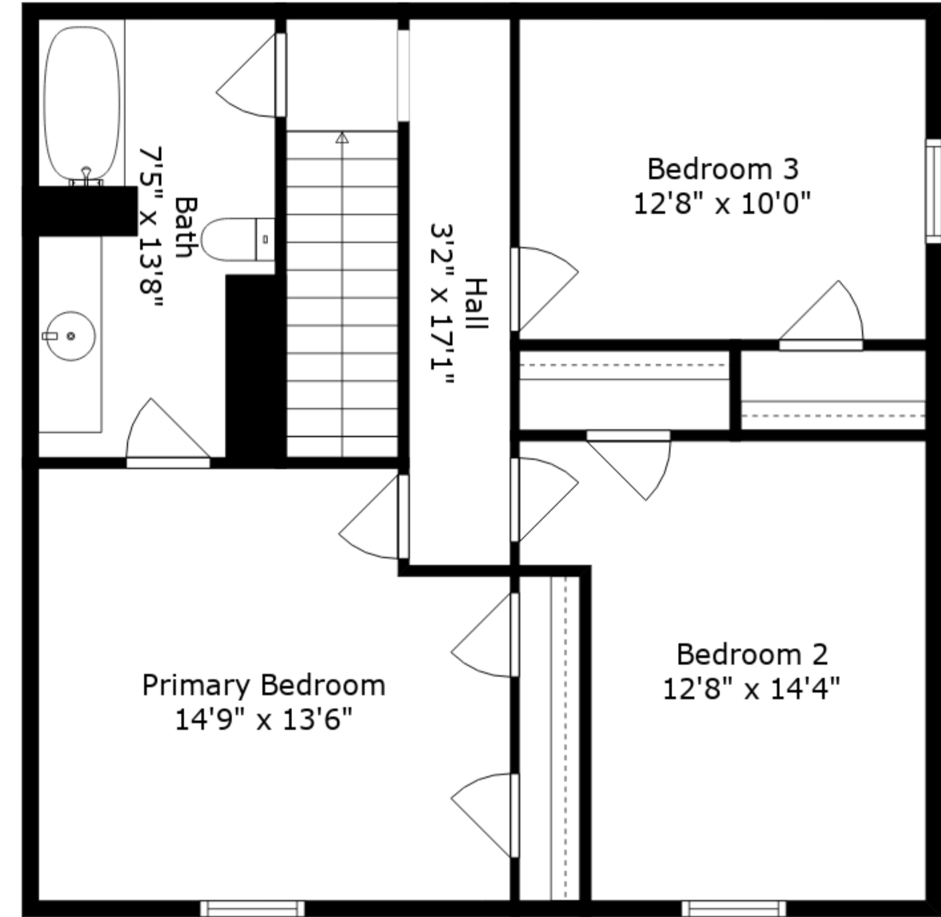
Upper Floor
