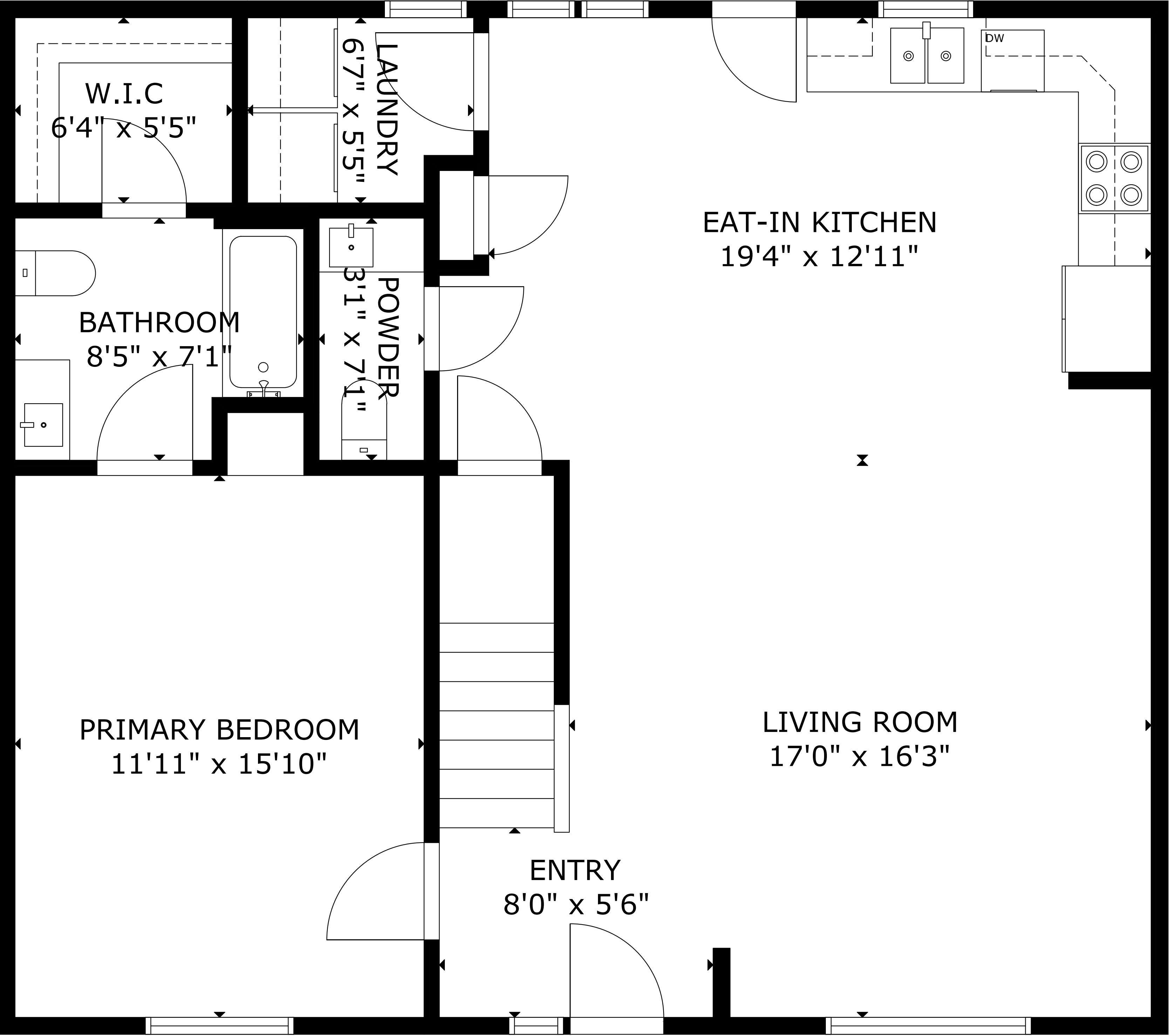
MAIN FLOOR
