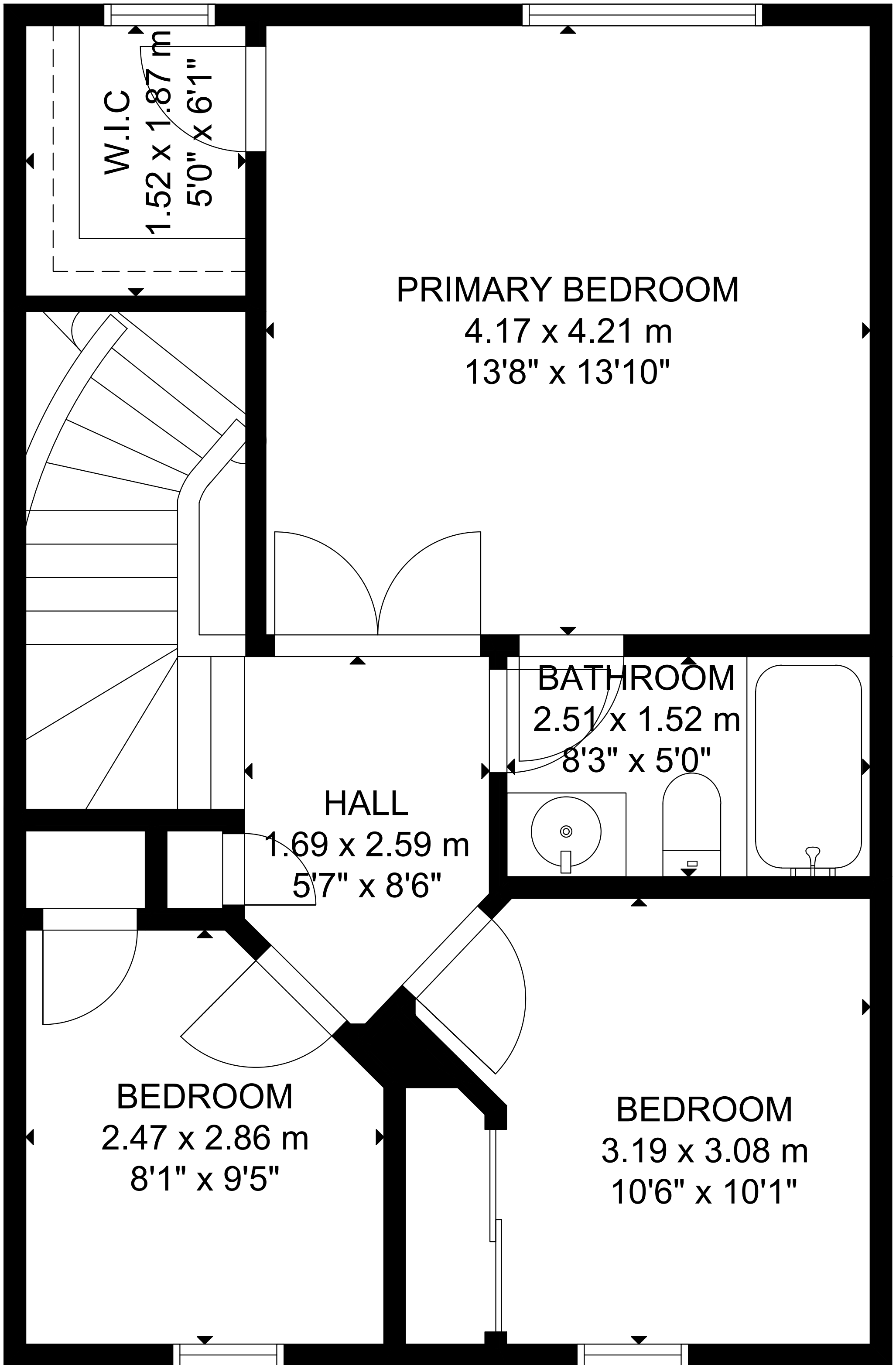
SECOND FLOOR
