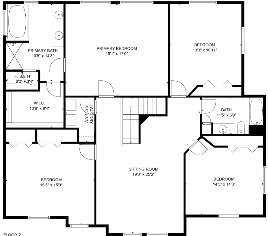
FLOOR 2
